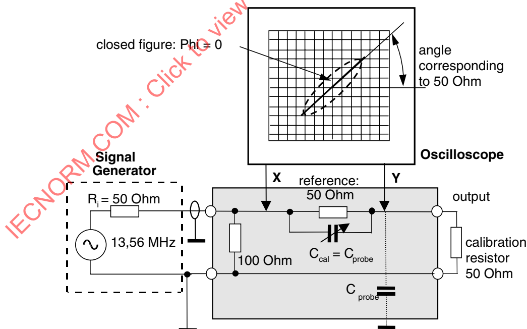
Figure B.1 — Calibration set-up (Step 1)
