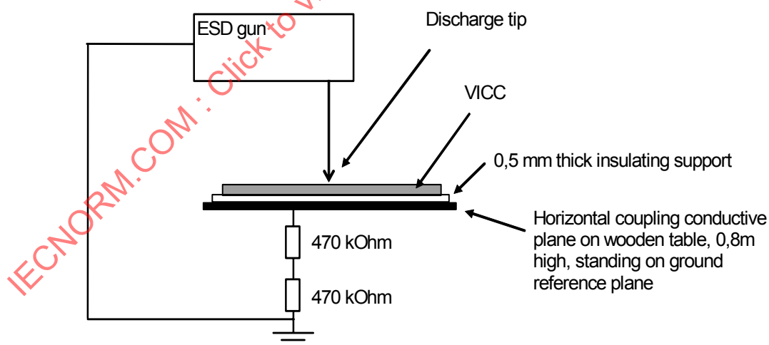
Figure 1 — ESD test circuit
