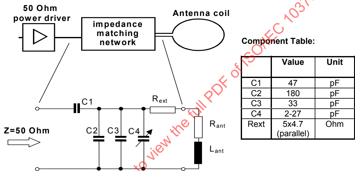
Figure A.3 — Impedance matching network
