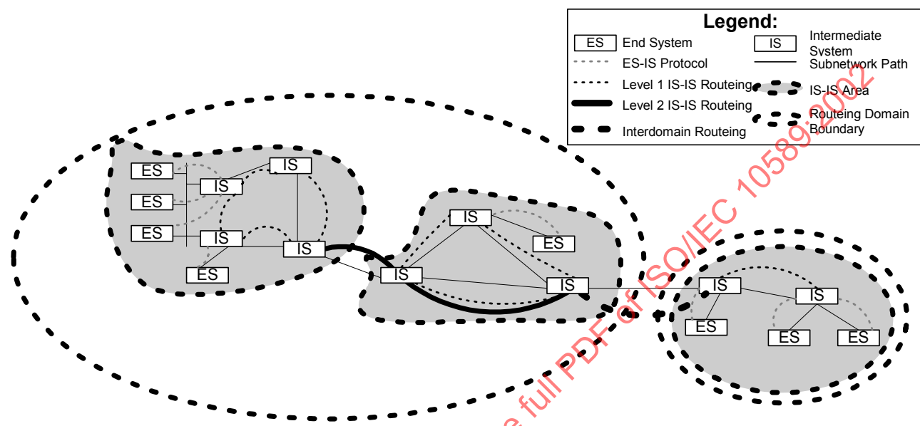
Figure 2 Topologies and Systems supported by Intradomain Routing
