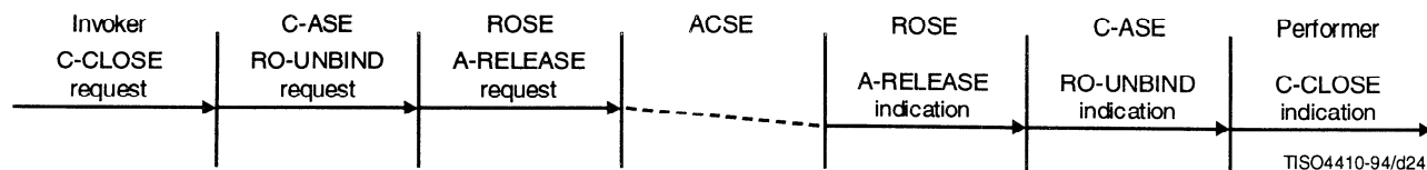
Figure 24 – Realization of an unbind using ACSE services
