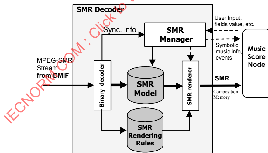
Figure 2 — MPEG SMR DECODER
