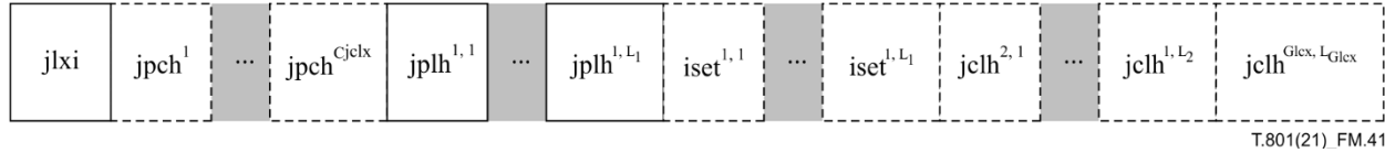
Figure M.41 – Organization of the contents of a Compositing Layer Extensions box
