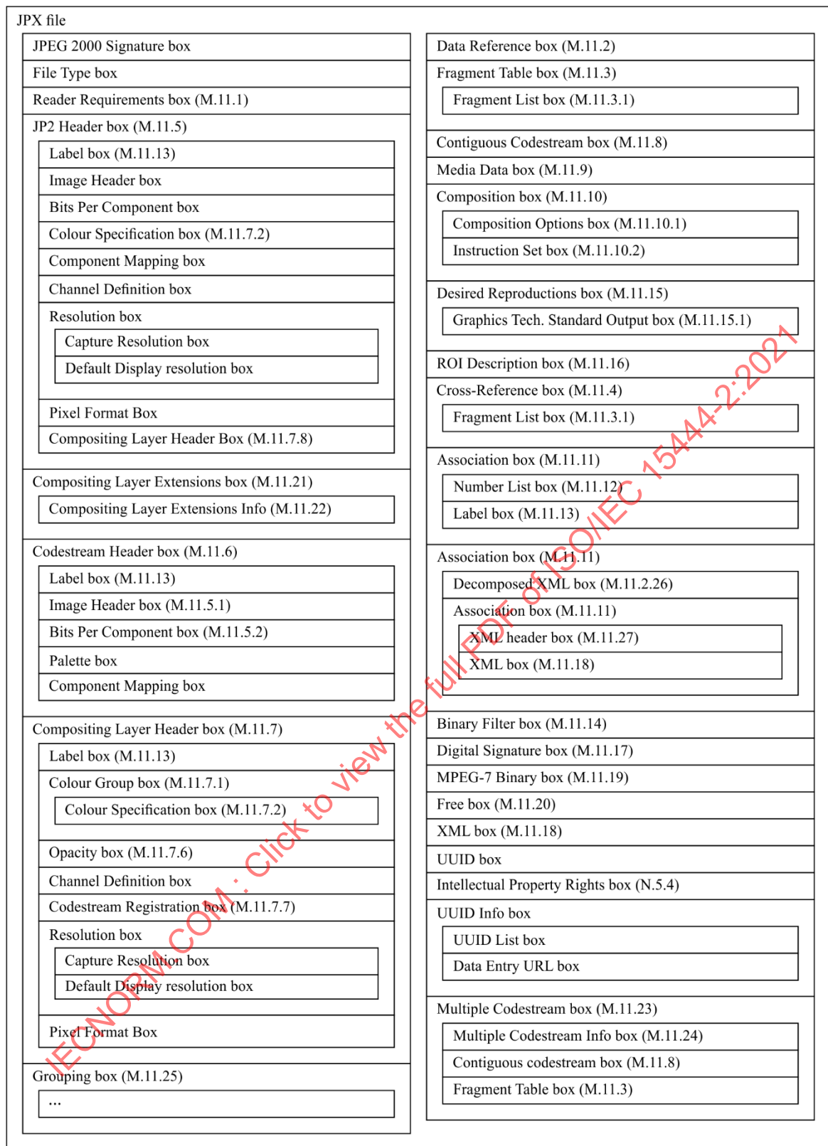
Figure M.6 – Boxes defined within a JPX file
