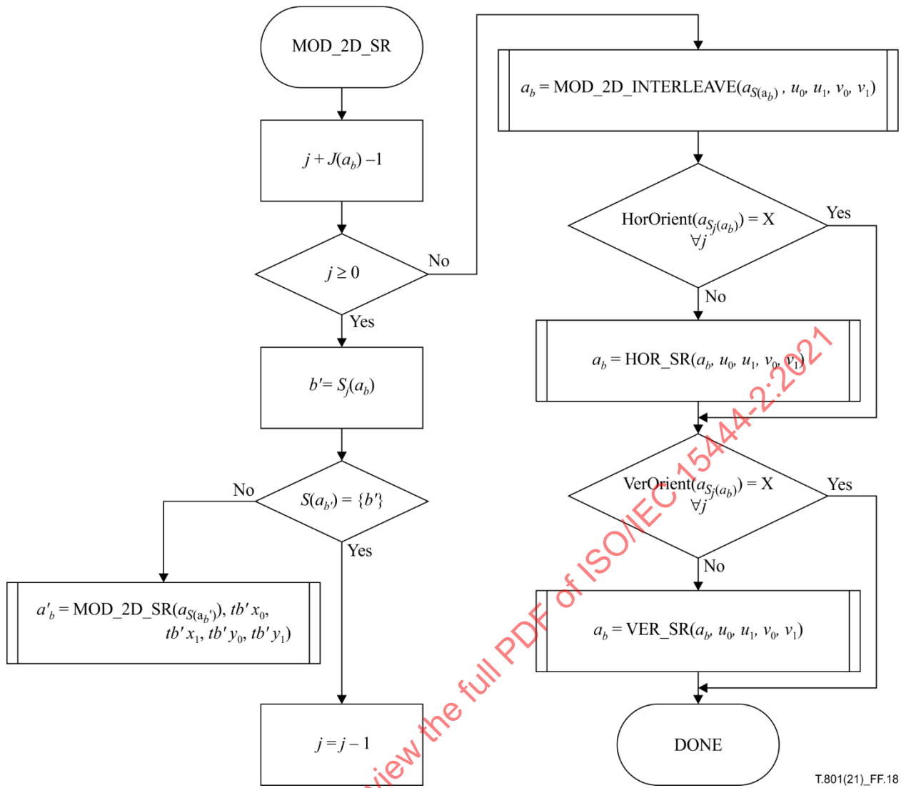
Figure F.18 – The MOD_2D_SR procedure
