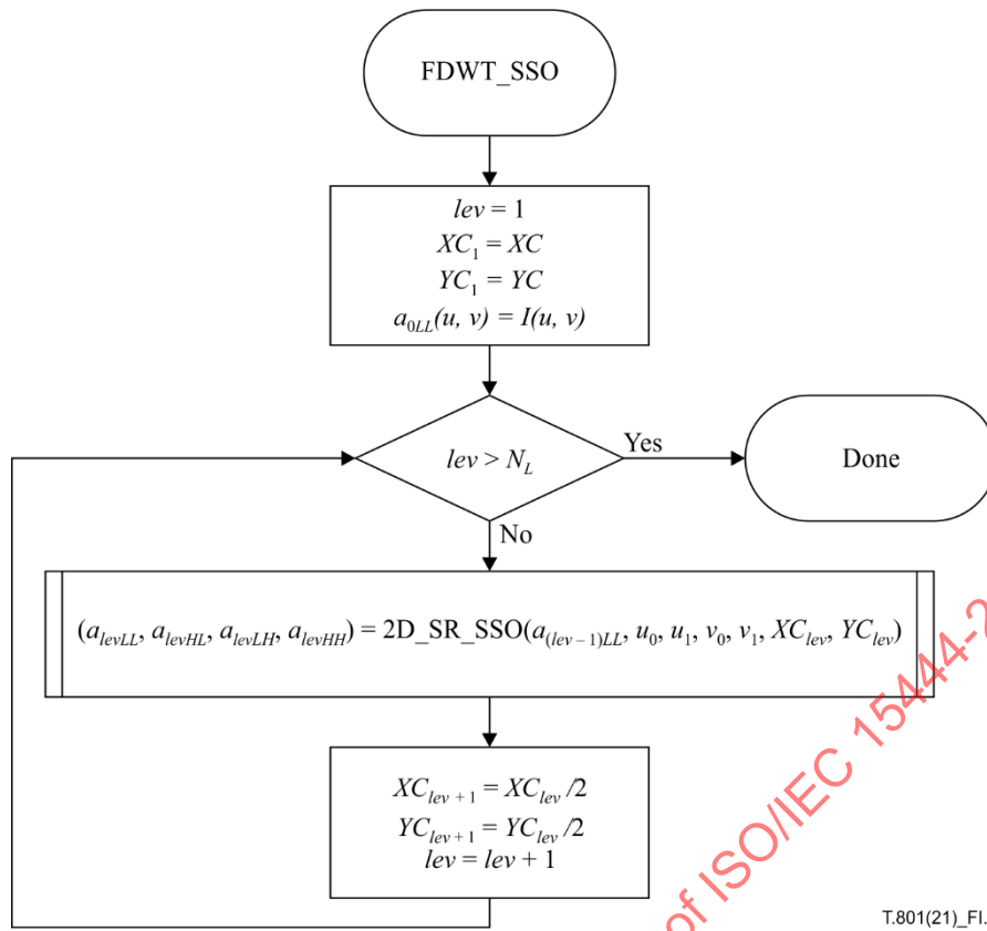
Figure I.6 – The FDWT_SSO procedure
