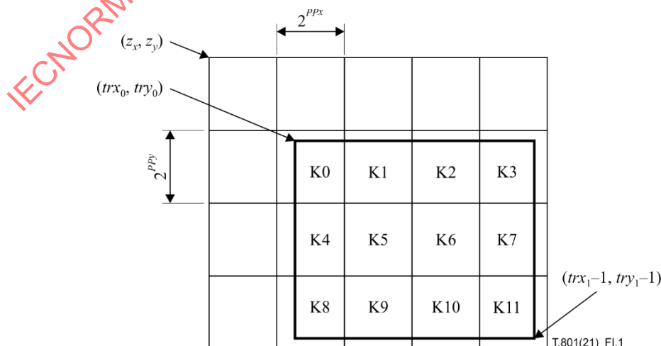
Figure I.1 – Precincts of one reduced resolution (modified Figure B.8 of Rec. ITU-T T.800 | ISO/IEC 15444-1)
