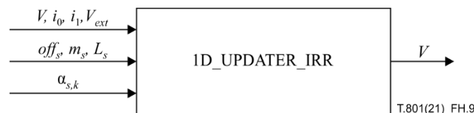
Figure H.9 – Parameters of the 1D_UPDATER_IRR procedure
