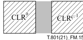
Figure M.15 – Organization of the contents of a Colour Group box
