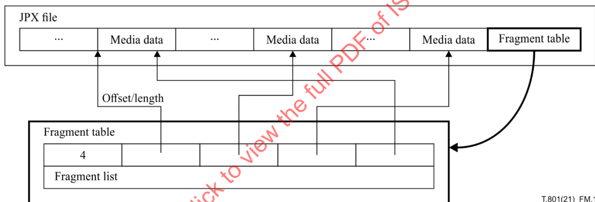
Figure M.1 – Example fragmented JPX file where all fragments are in the same file
