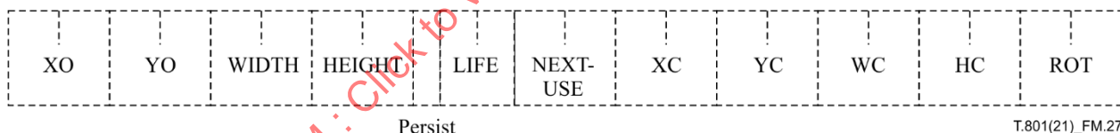
Figure M.27 – Organization of the contents of an INST field within an Instruction Set box
