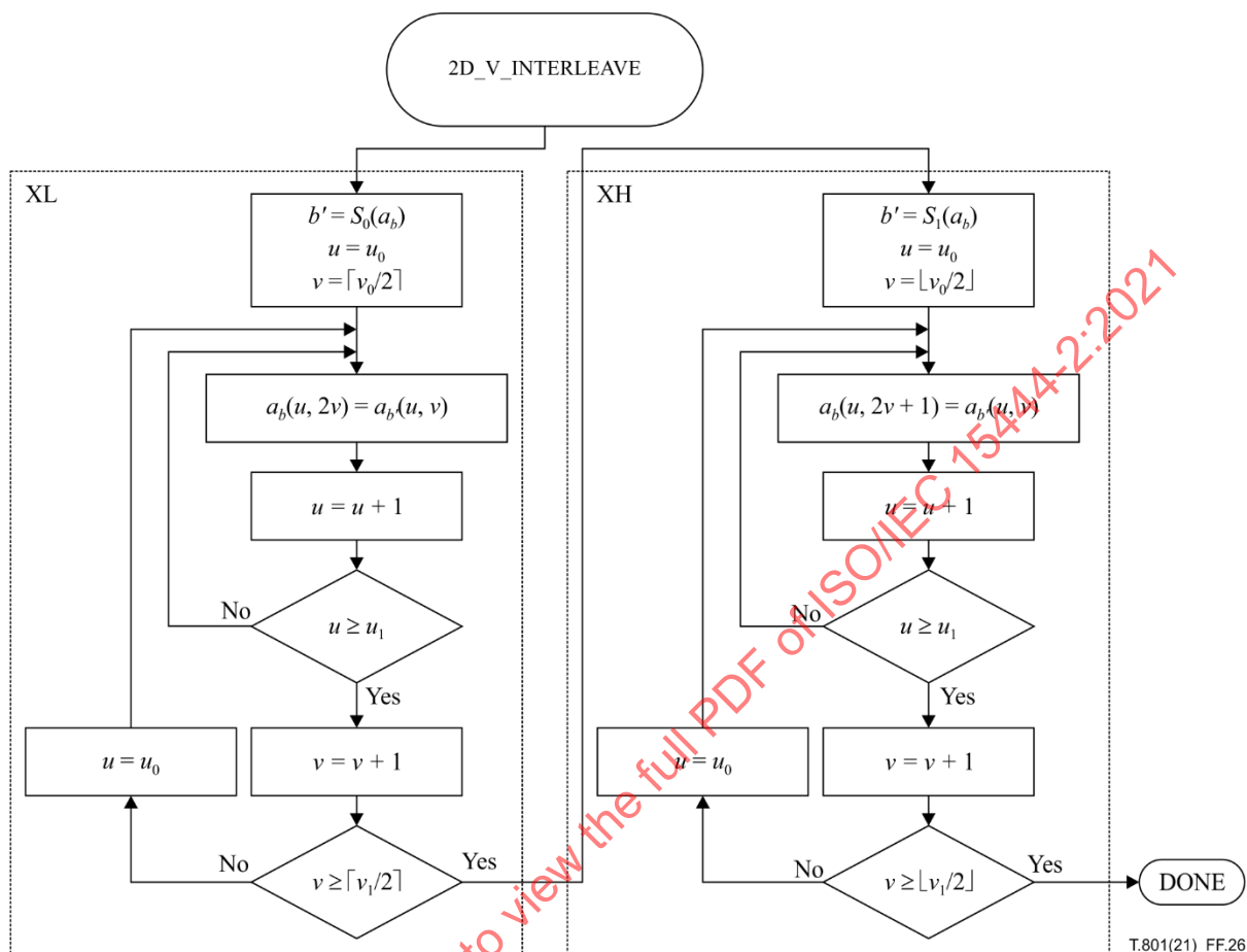
Figure F.26 – The 2D_V_INTERLEAVE procedure
