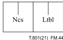
Figure M.44 – Organization of the contents of a Multiple Codestream Offsets box
