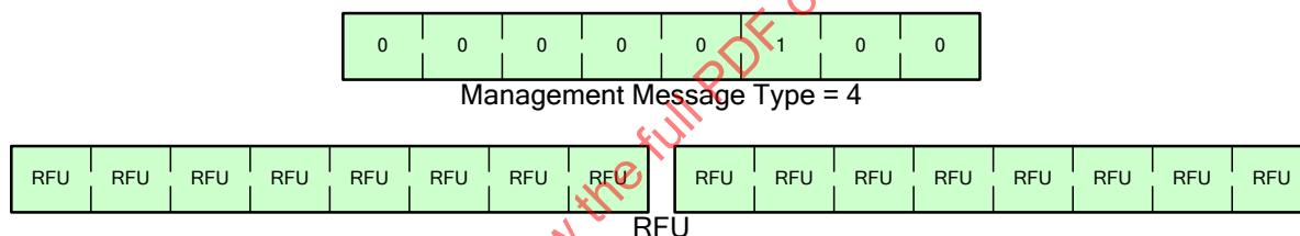
Figure 15 — DAS-REQ message format
