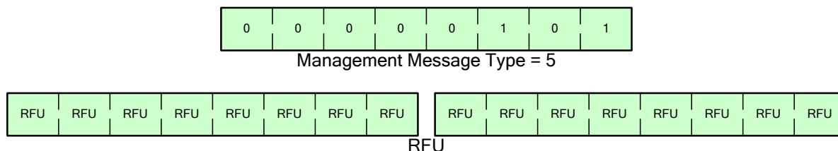
Figure 16 — DAS-RSP message format
