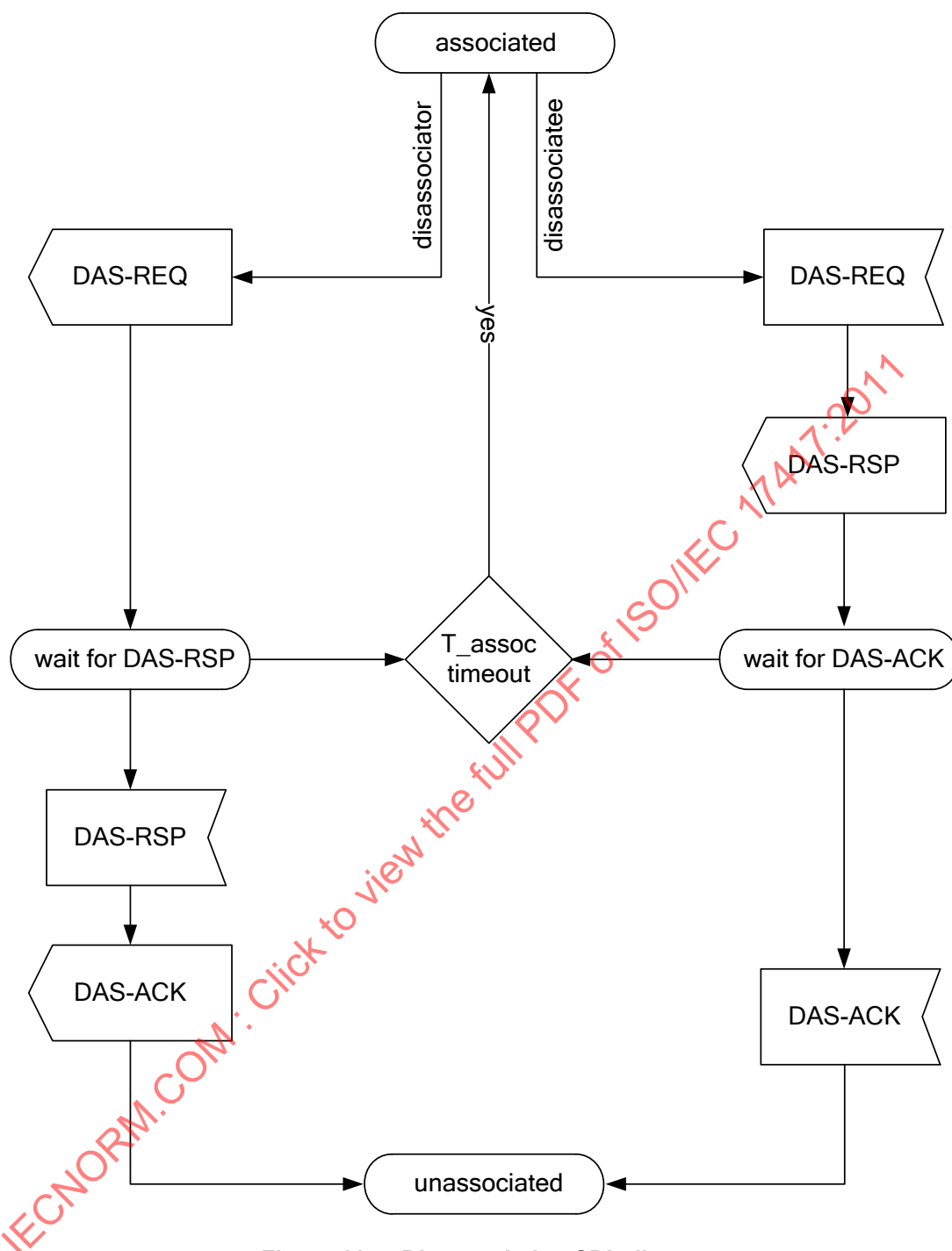
Figure 11 — Disassociation SDL diagram
