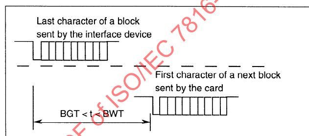
Figure 21 — Block waiting time and block guardtime
