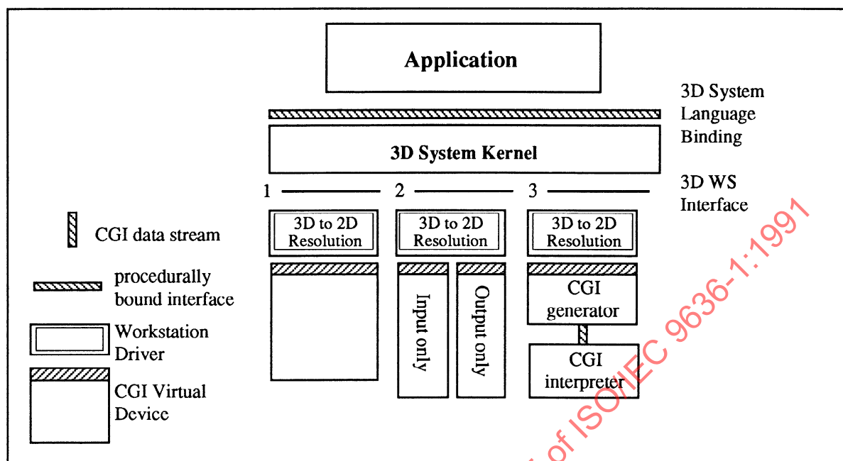
Figure 4 – CGI Virtual Devices as 3D workstations
