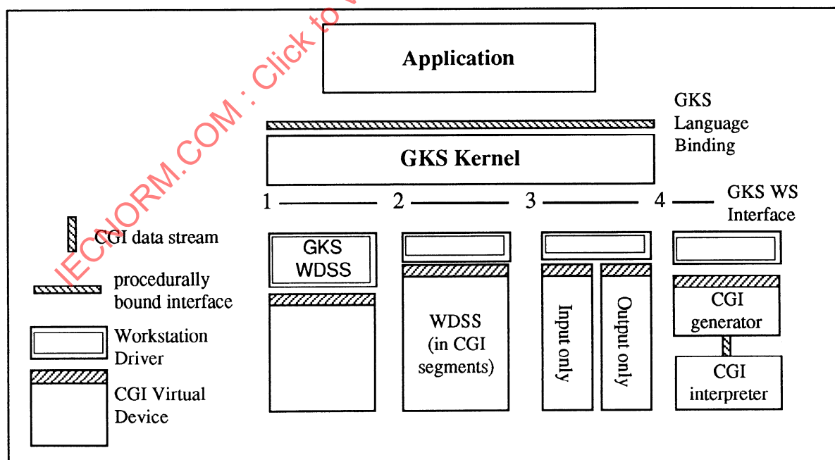
Figure 2 – CGI Virtual Devices as GKS workstations
