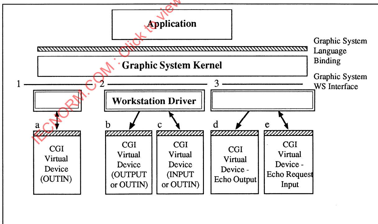
Figure 5 – Implementing input/output workstations as combinations of CGI Virtual Devices
