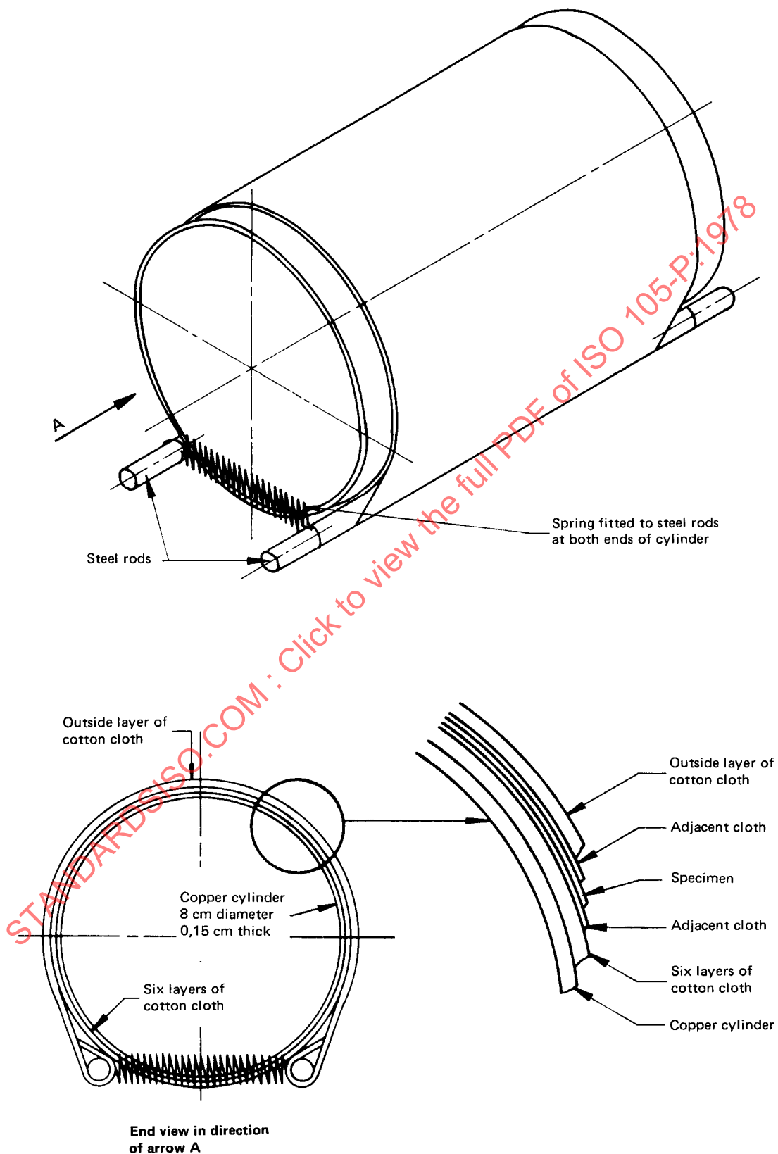
FIGURE 1 — Specimen holder
