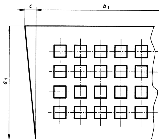
Figure 3 — Measurement of amount out-of-square
