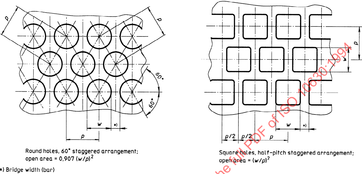
Figure 1 — Examples of hole arrangements
