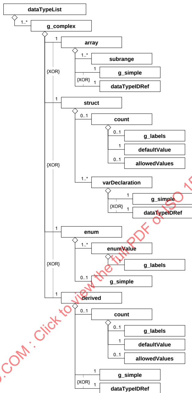
Figure G.5 — dataTypelList
