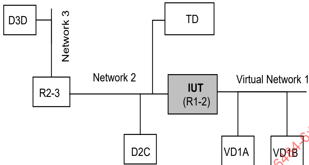
Figure 10-4. Logical internetwork configuration for virtual routing functionality tests.
