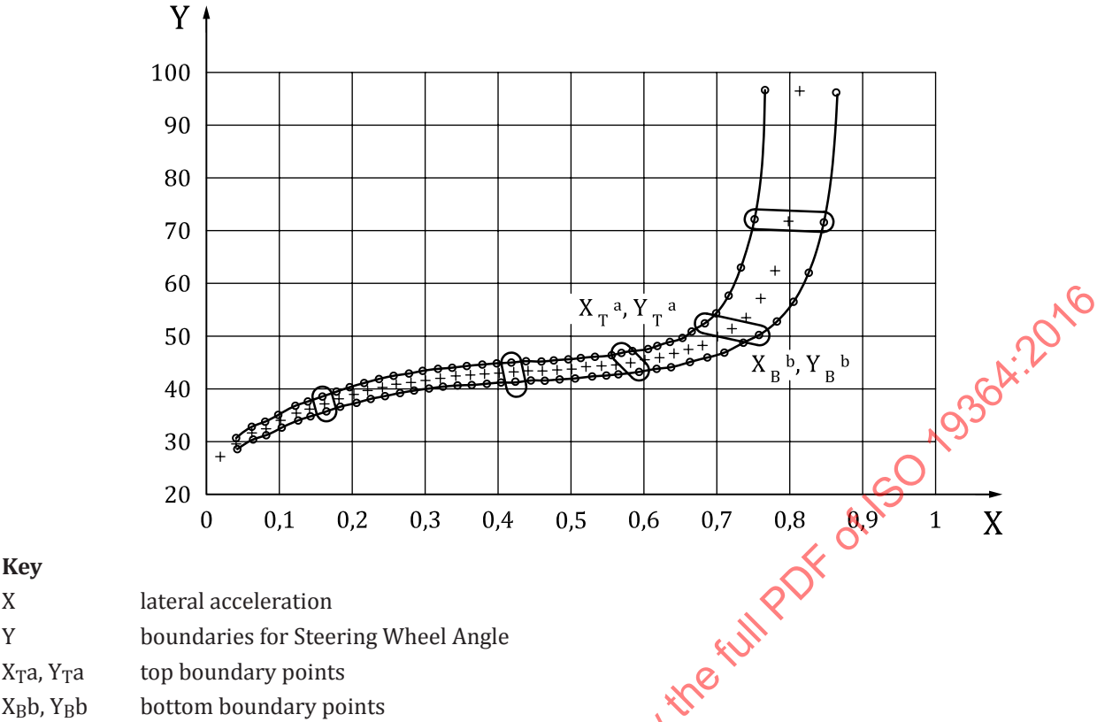
Figure 1 — Steer vs. lateral acceleration boundaries for an example simulation with limit understeer
