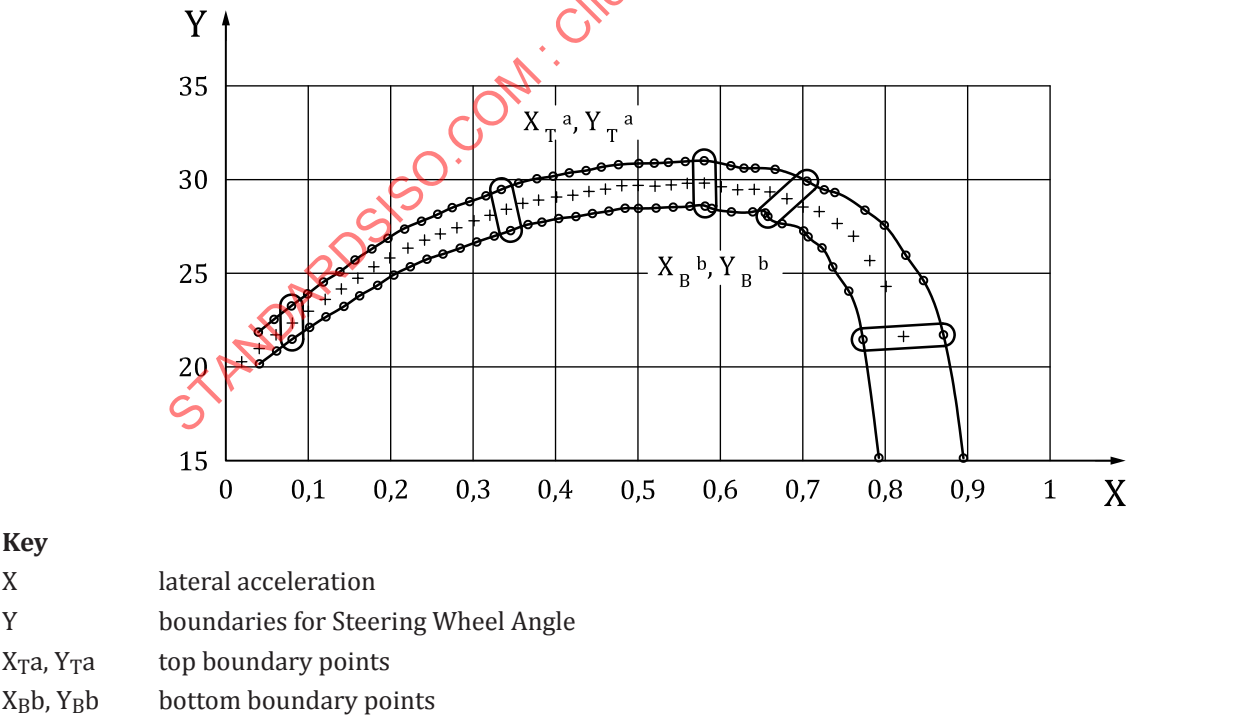
Figure 2 — Steer vs. lateral acceleration boundaries for an example simulation with limit oversteer
