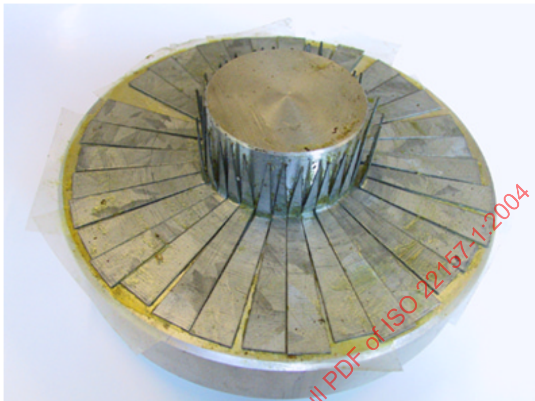
Figure 2 — Intermediate layer
