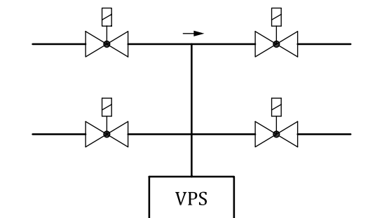
a) External valves supervised by a VPS
