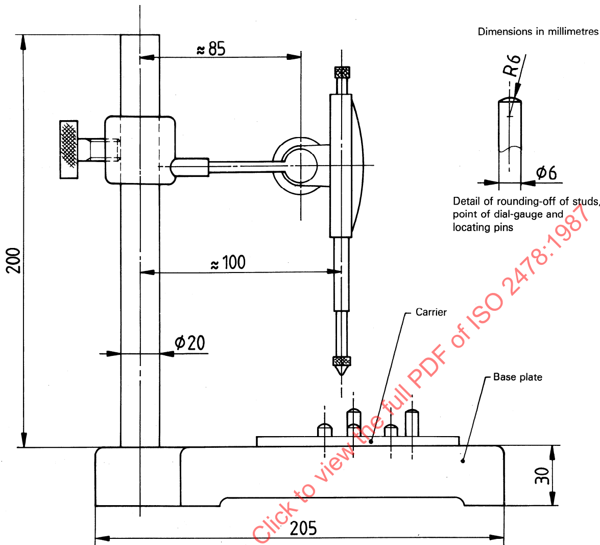
Figure 1 — Length-measuring device
