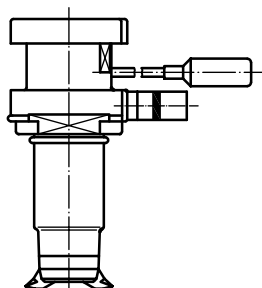
d) Nozzle for lateral injection
