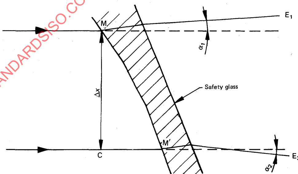
FIGURE — Diagrammatic representation of optical distortion
