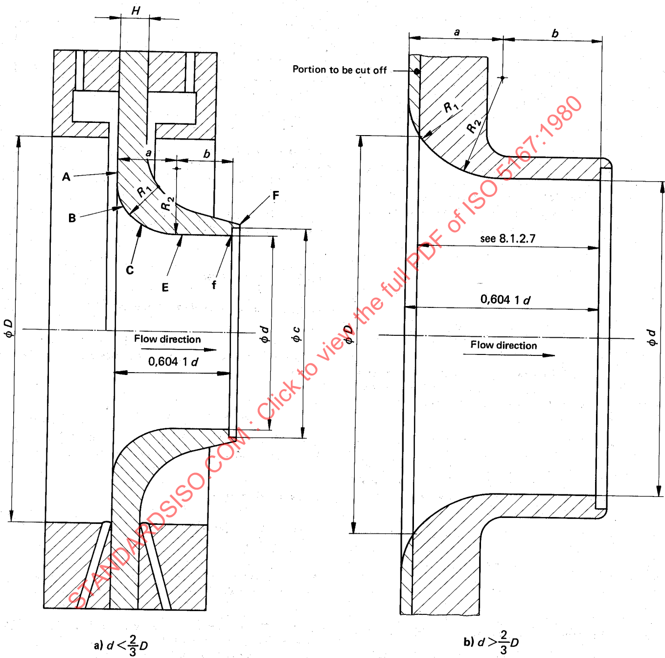
FIGURE 5 – ISA 1932 nozzle
