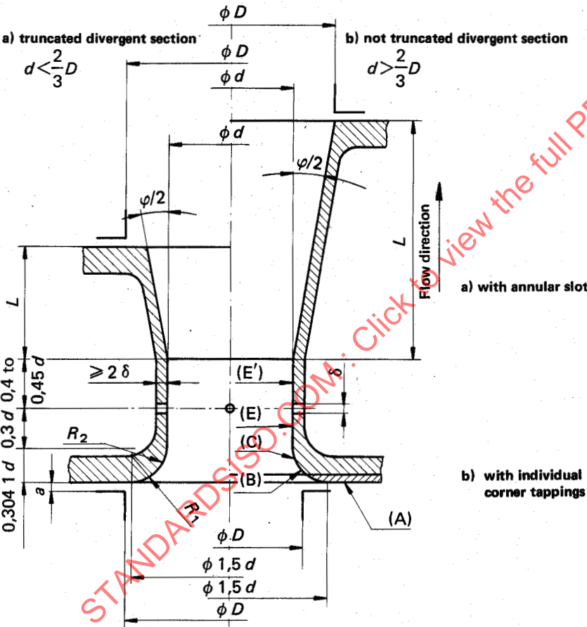
FIGURE 9 – Venturi nozzle
