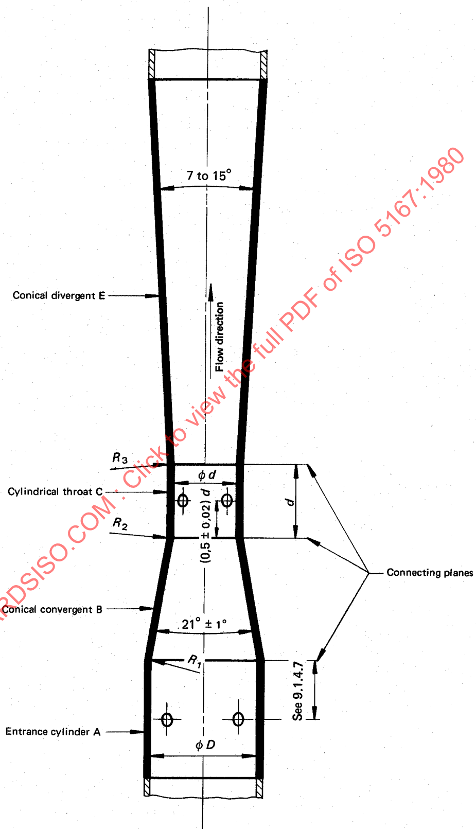
FIGURE 7 — Geometric profile of the classical venturi tube
