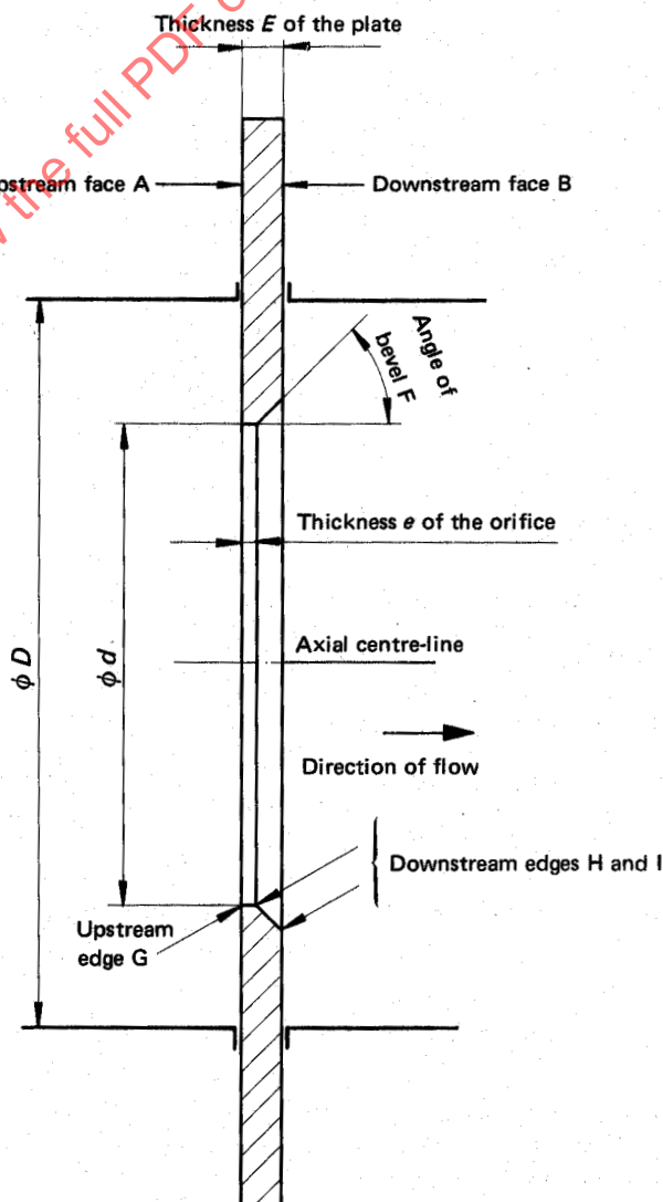
FIGURE 2 — Standard orifice plate
