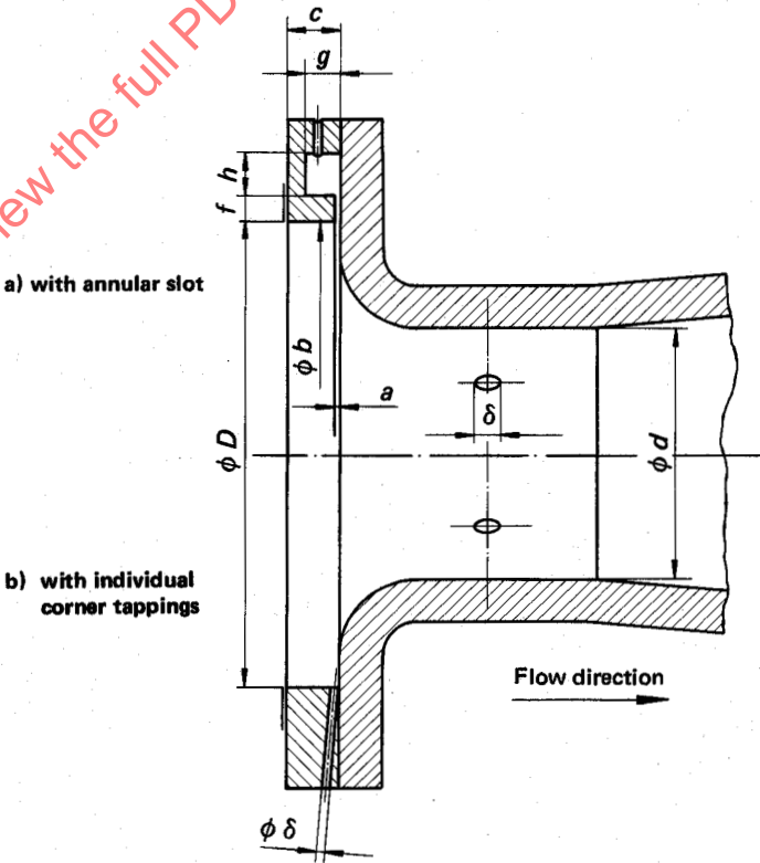
FIGURE 10 – Carrier ring
