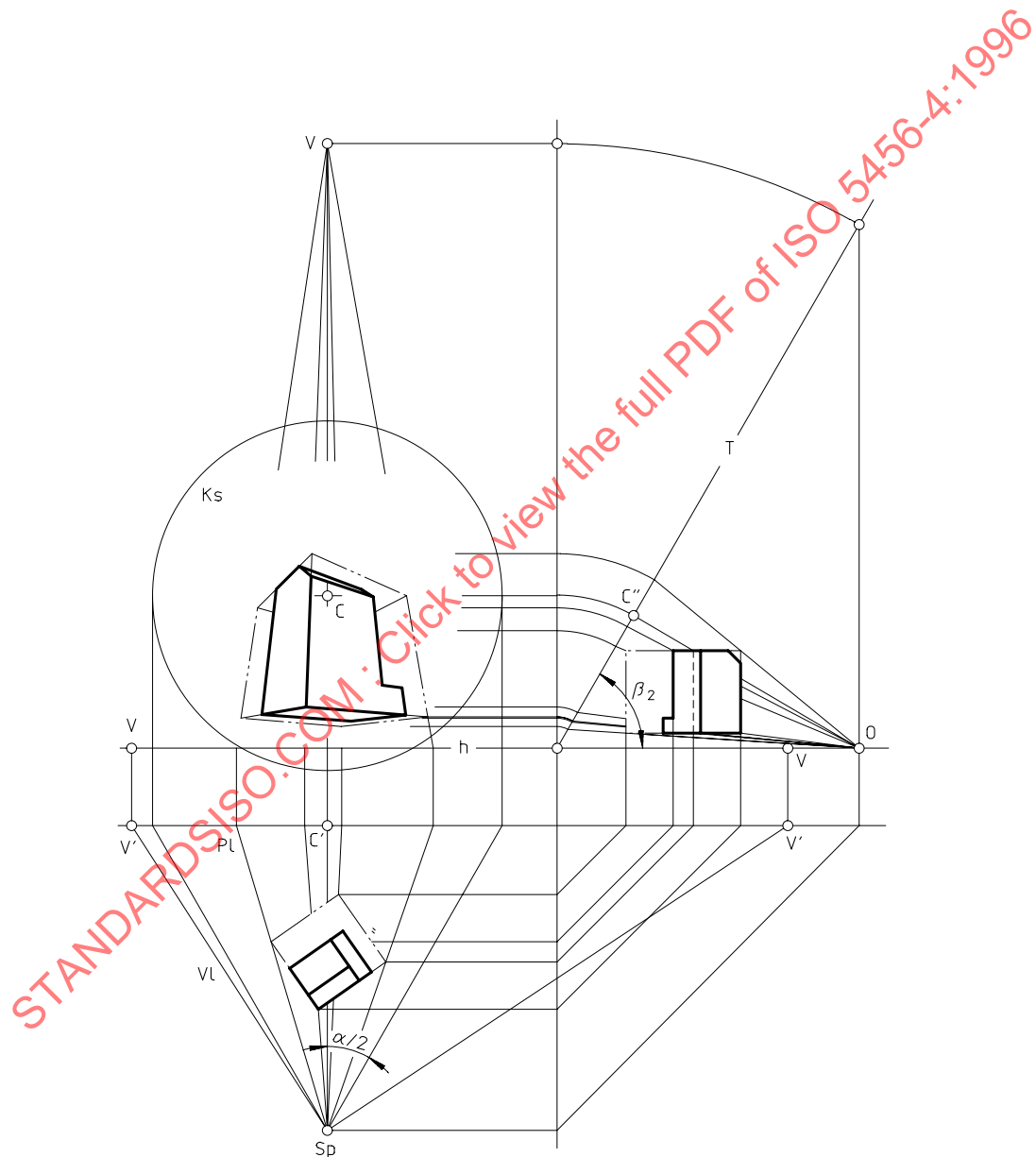
Figure 15 — Object, framed in a cube (indicated by a double-dashed line), in front of a projection plane inclined towards the projection centre
