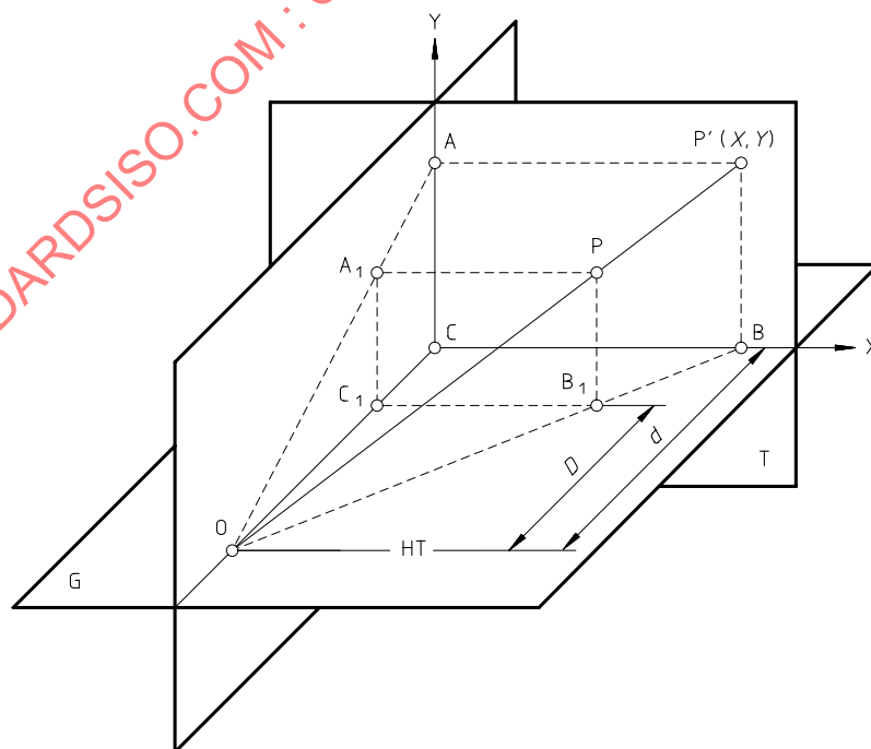
Figure 17 — Coordinate piercing method
