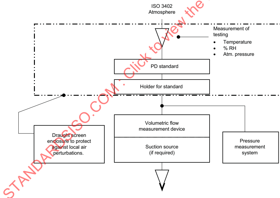
Figure A.2 — Typical arrangement of calibration apparatus
