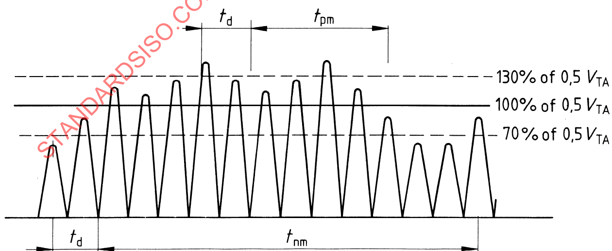
Figure 7 — Modulation tests
