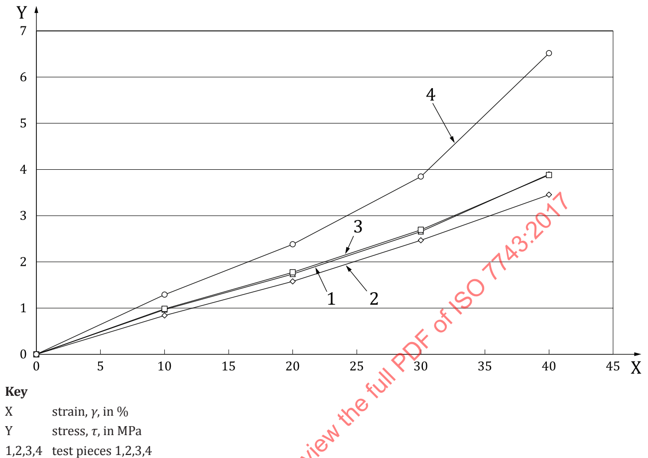
Figure A.2 — Static stress-strain properties in compression — Bonded test pieces — Stresses presented without any correction
