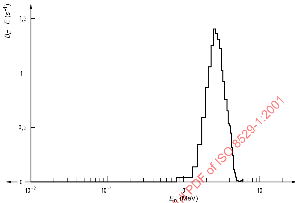
Figure A.3 — Neutron spectrum from a ^{241}\text{AmB}(\alpha, n) source
