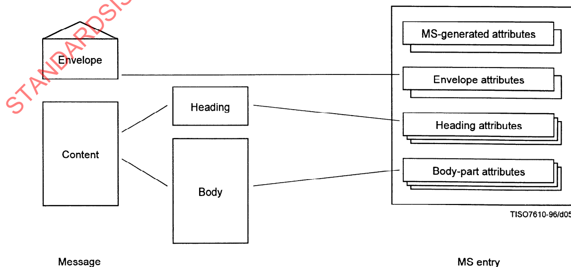
Figure 5 – Mapping an IPM to an MS entry
