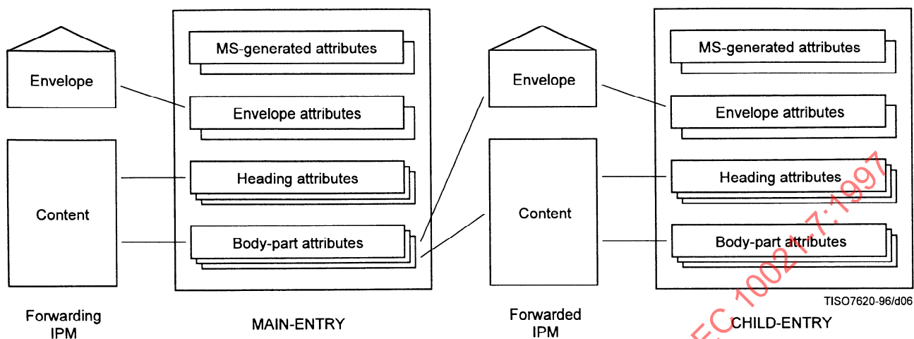
Figure 6 – Mapping a Forwarding message to an IPMS-MS entry
