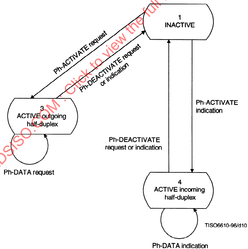
Figure 9 – State transition diagram for half-duplex mode
