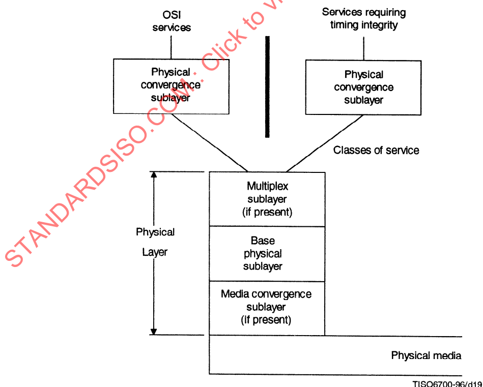
Figure A.1 – Structure of the Physical Layer
