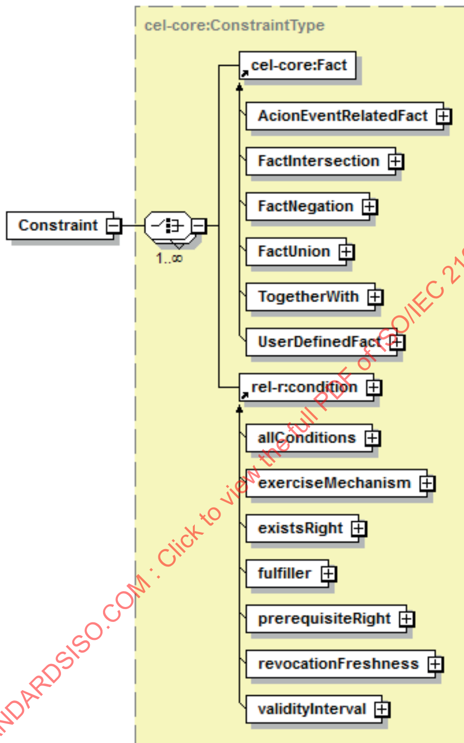
Figure 23 — Constraint element
