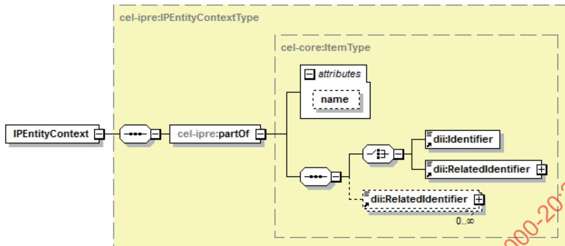
Figure 37 — IPEntityContext constraint
