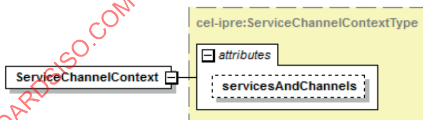
Figure 38 — ServiceChannelContext constraint
