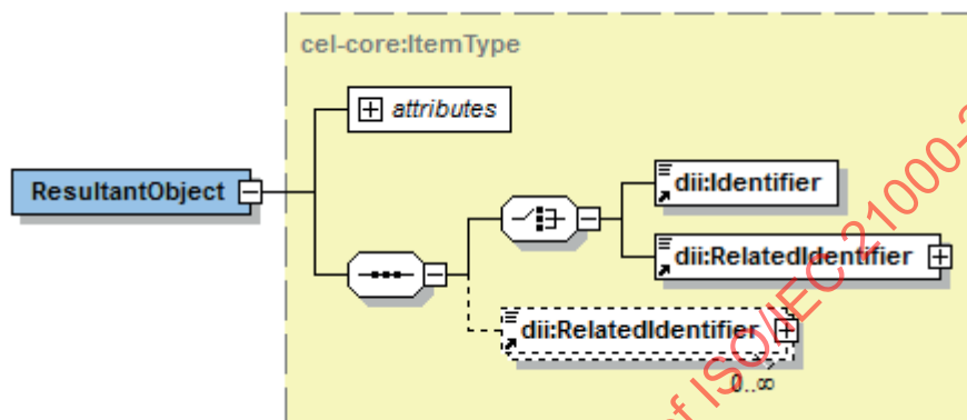
Figure 22 — ResultantObject element
