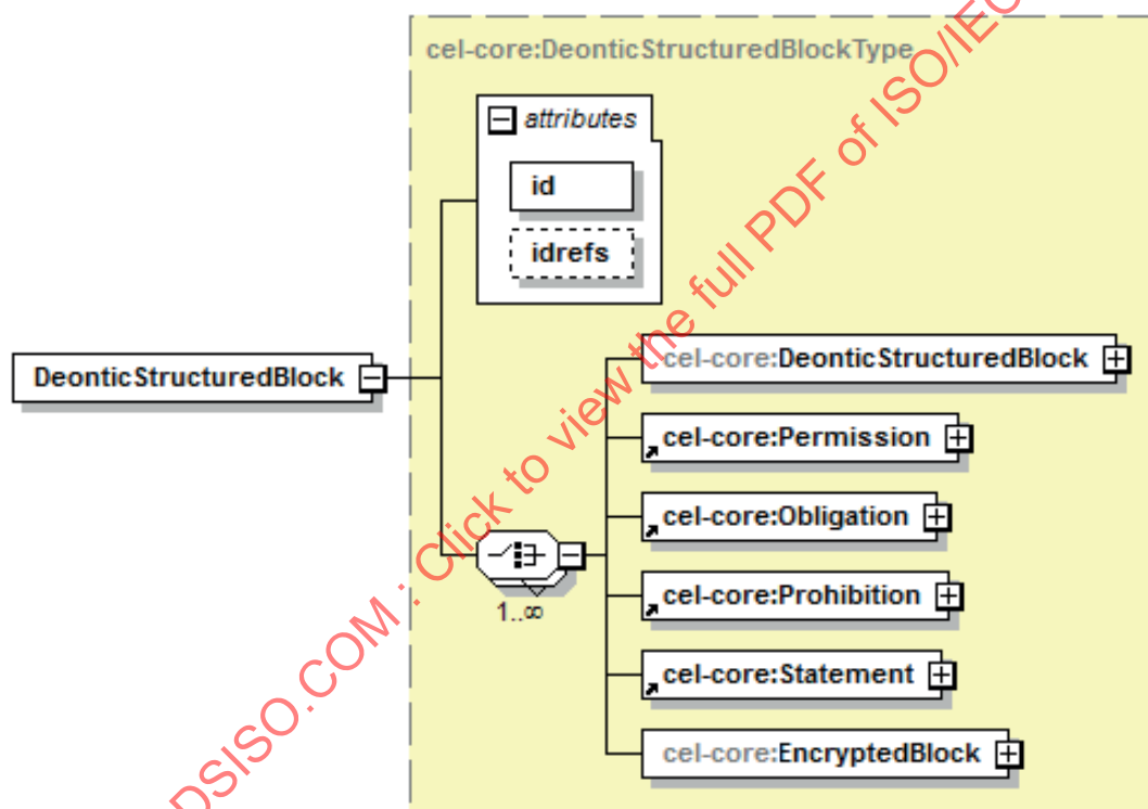
Figure 11 — DeonticStructuredBlock element
