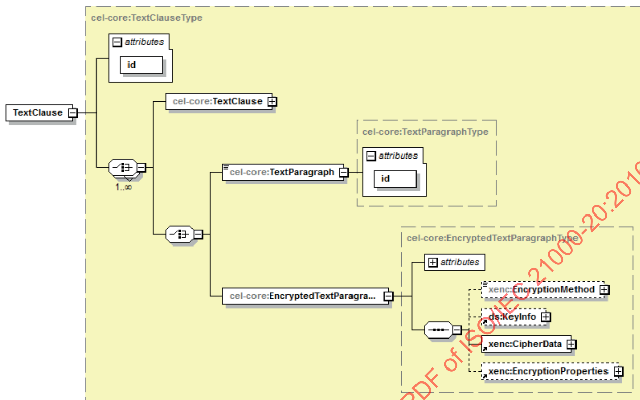
Figure 9 — TextClause element
