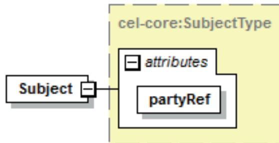
Figure 16 — Subject element
