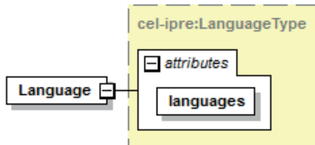
Figure 35 — Language constraint
