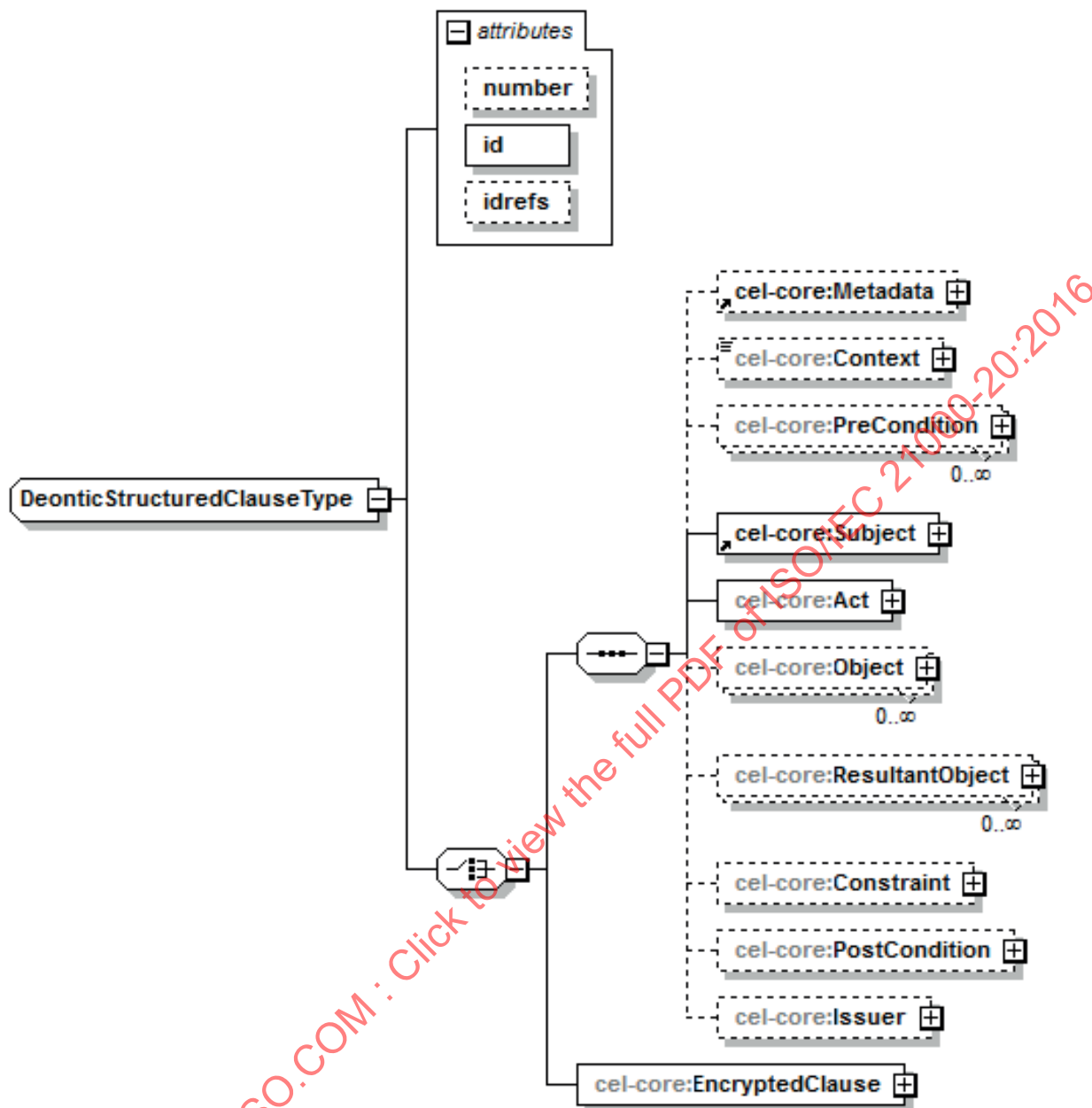
Figure 12 — DeonticStructuredClauseType type
