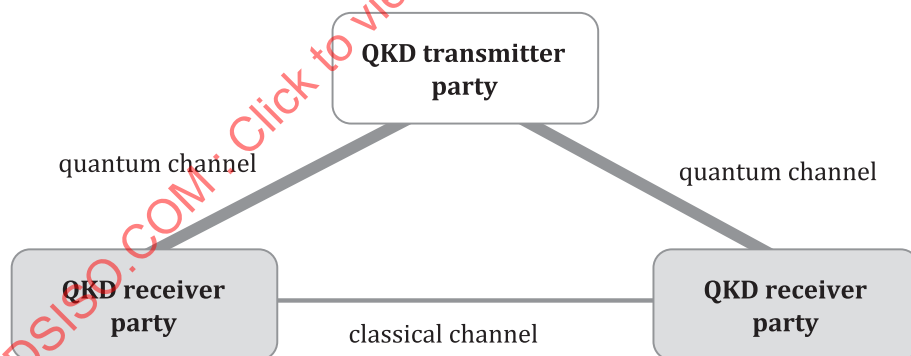
Figure 3 — EB-QKD protocol
