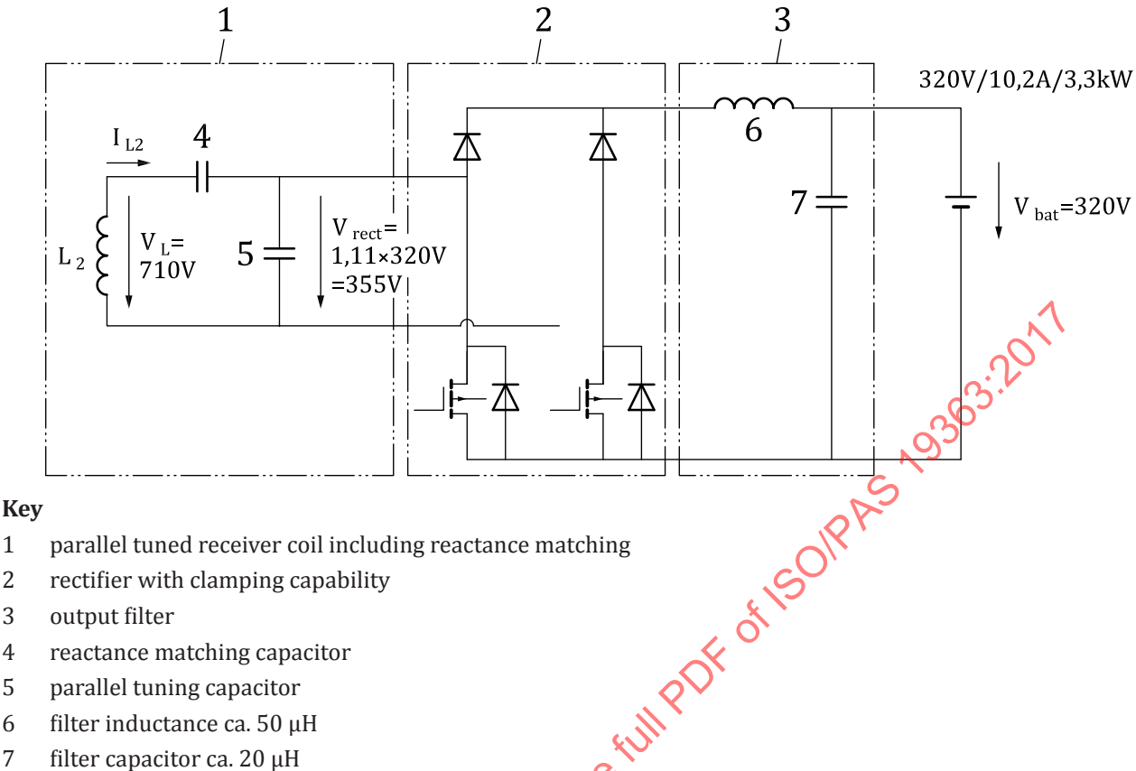
Figure B.3 — Schematics of power electronics for the MF-WPT1/Z1 DD reference EV device
