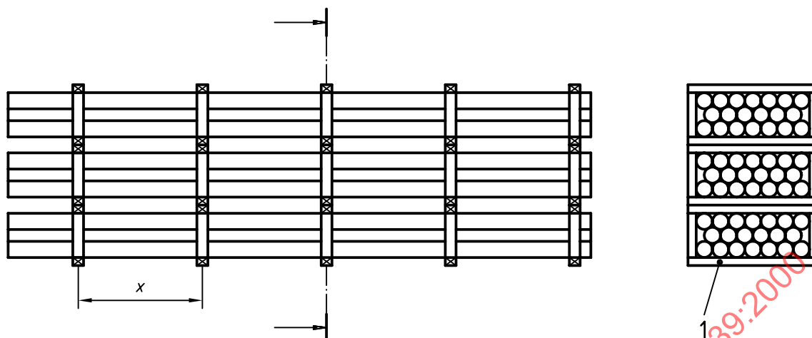
Figure 15 — Support frame
