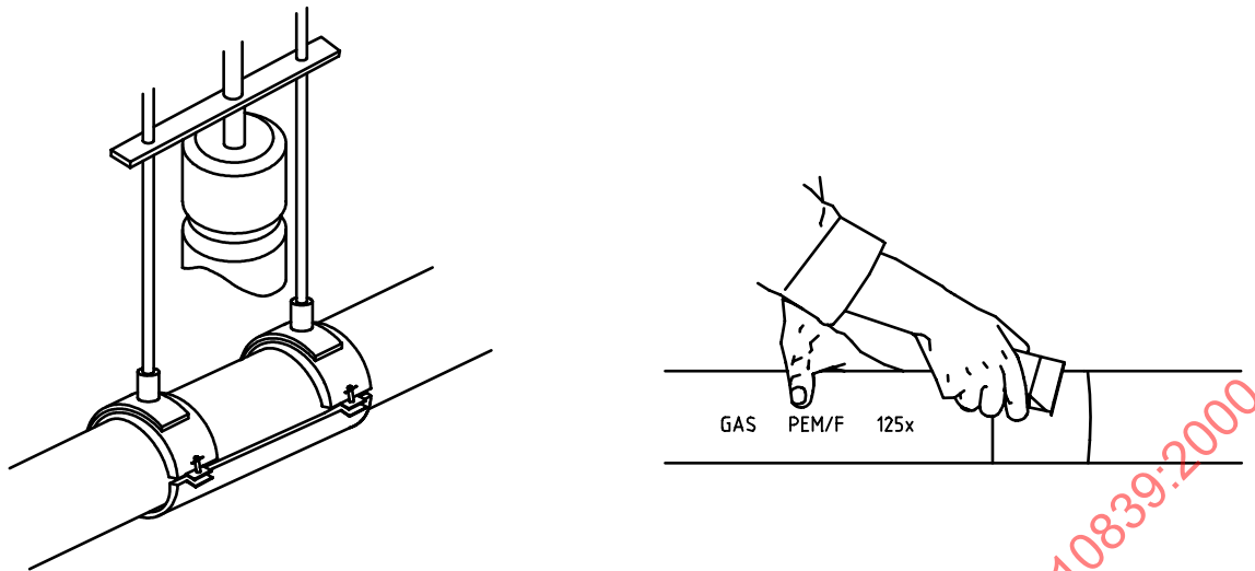
Figure 11 — Surface scraping
