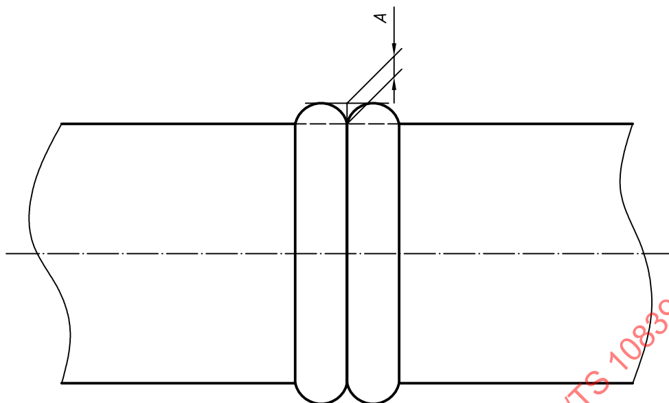
Figure 16 — Bead symmetry
