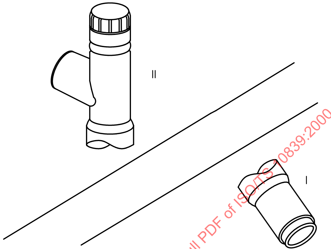
Figure 10 — Type I and II saddle fusion fittings
