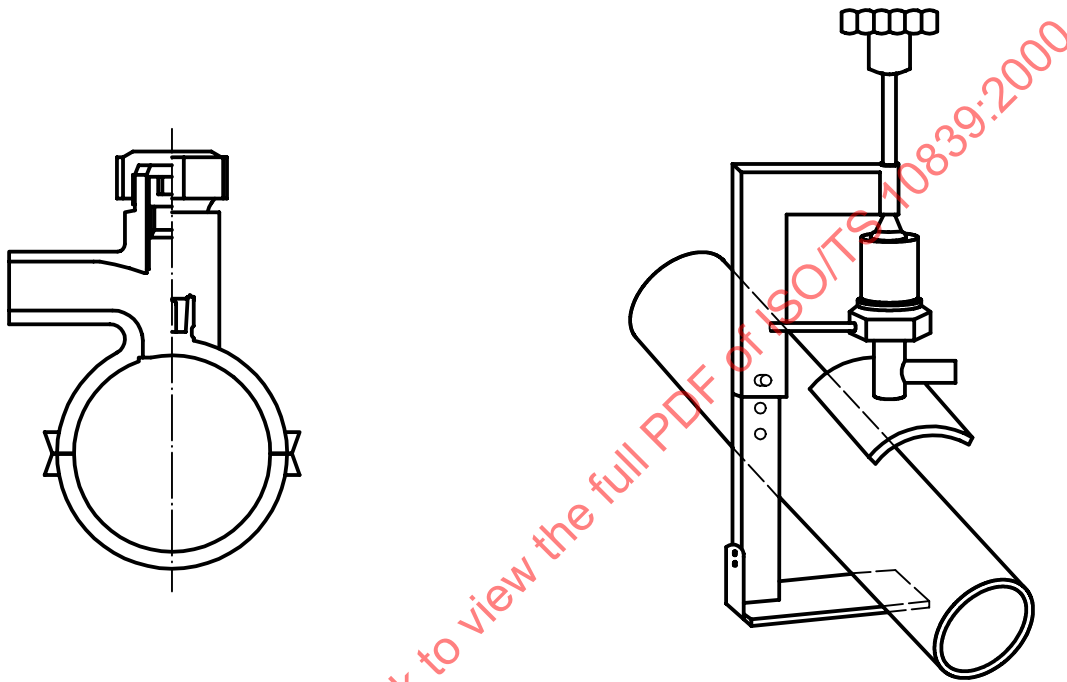
Figure 14 — Example of installation of a saddle
