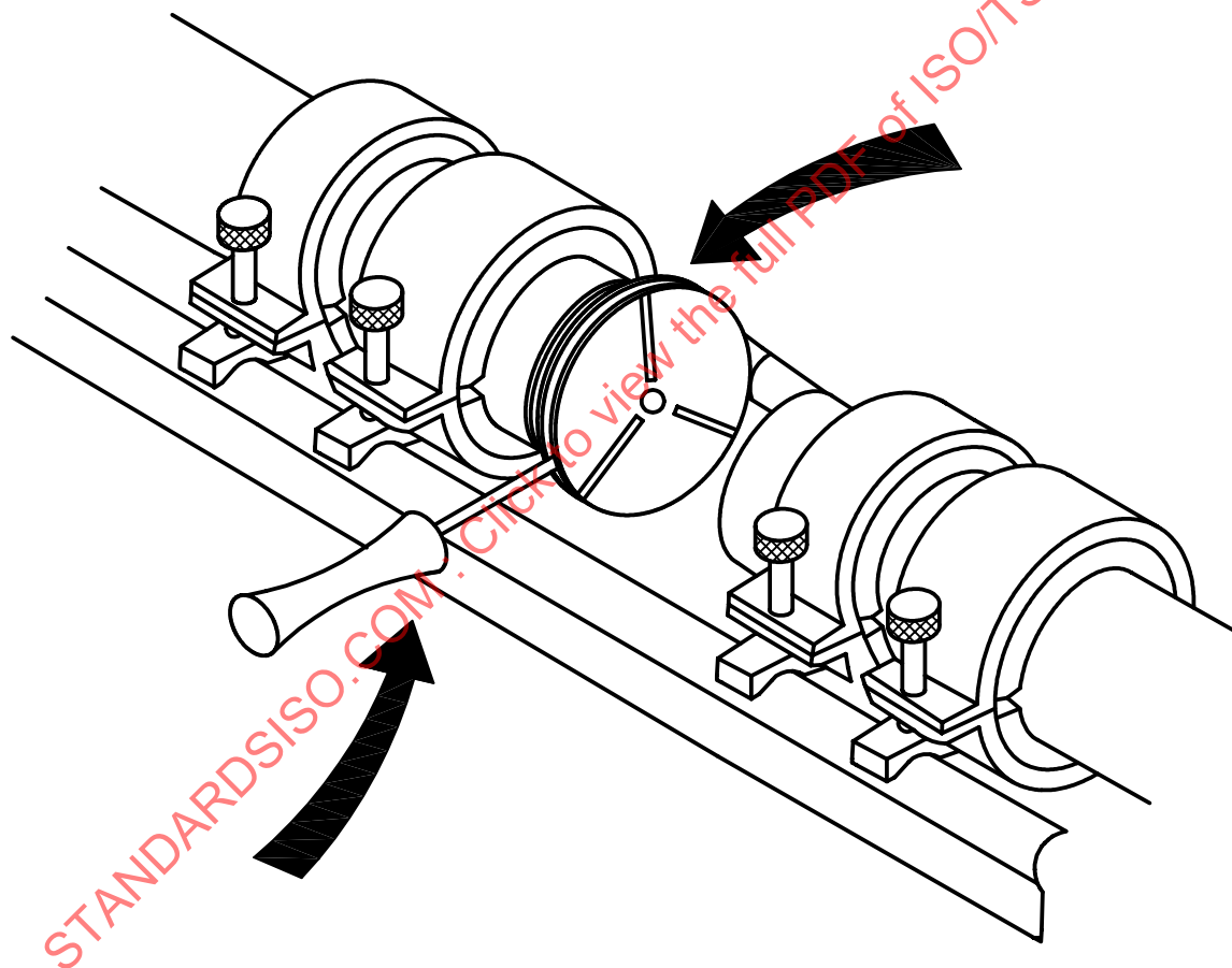
Figure 3 — Planing the spigot ends
