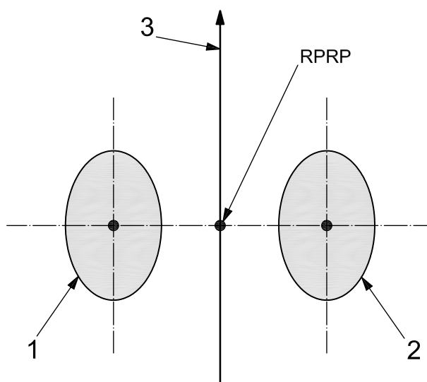
Figure B.2 — Definition of resonator pair symmetrical axis
