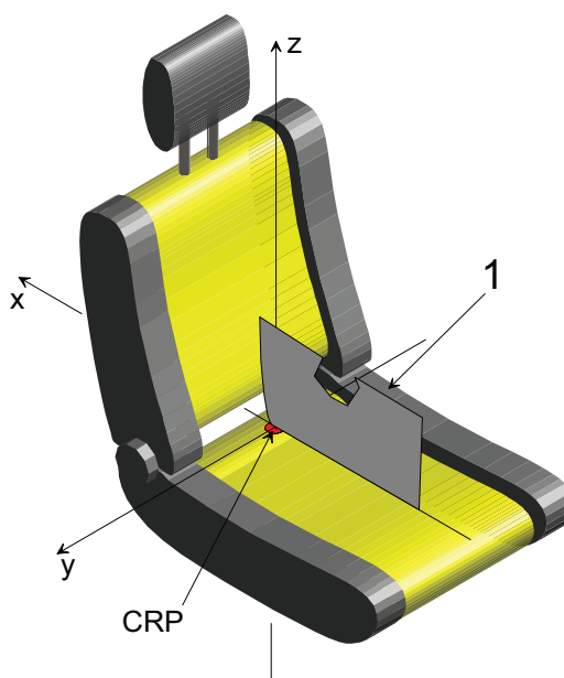
Figure B.4 — Reference co-ordinate system
