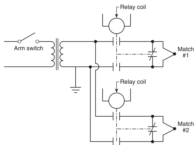
FIGURE A.8.3 Suggested Firing Circuit. Note that the relay contacts shown may be replaced by solid state switching devices. (Circuitry for test currents is omitted for clarity.)
