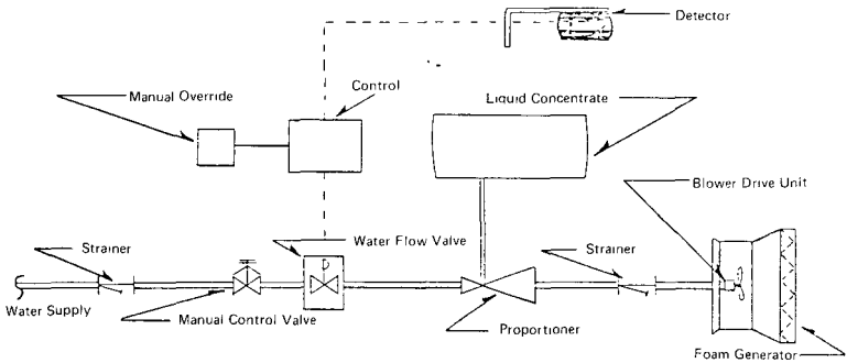
Figure A-1-9.5(a) Block Diagram of Automatic Medium or High Expansion Foam System.
