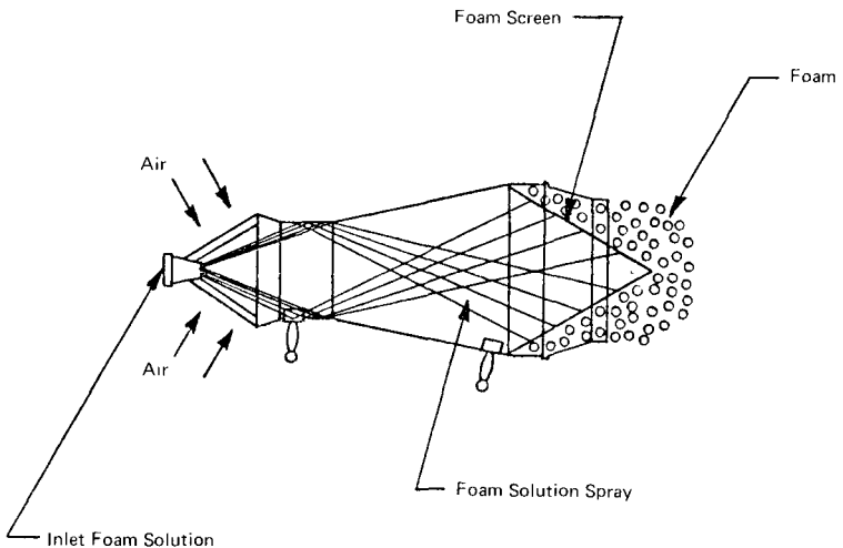
Figure A-1-9.5(b) Aspirating Type Foam Generator.
