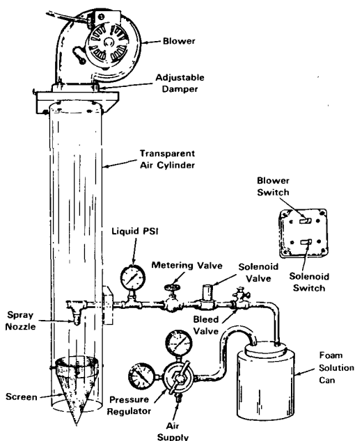
Figure A-1-10.5(b)(1) High Expansion Foam Quality Test Generator.
