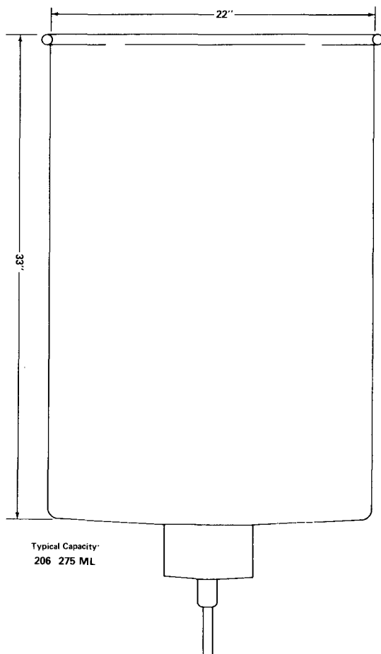
Figure A-1-10.5(b)(2) Typical Drainage Drum for High Expansion Foam Expansion and Drainage Test.
