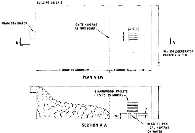
Figure A-1-10.5(a) Fire Performance Test.
