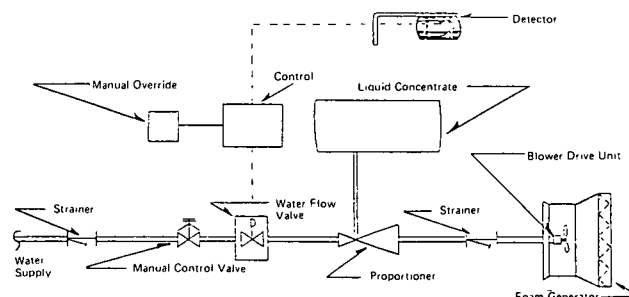
Figure A-1-9.5(a) Block Diagram of Automatic Medium- or High-Expansion Foam System.
