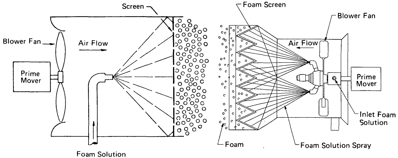
Figure A-1-9.5(c) Blower-type Foam Generators.
