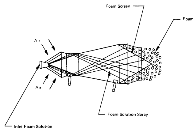
Figure A-1-9.5(b) Aspirating-type Foam Generator.
