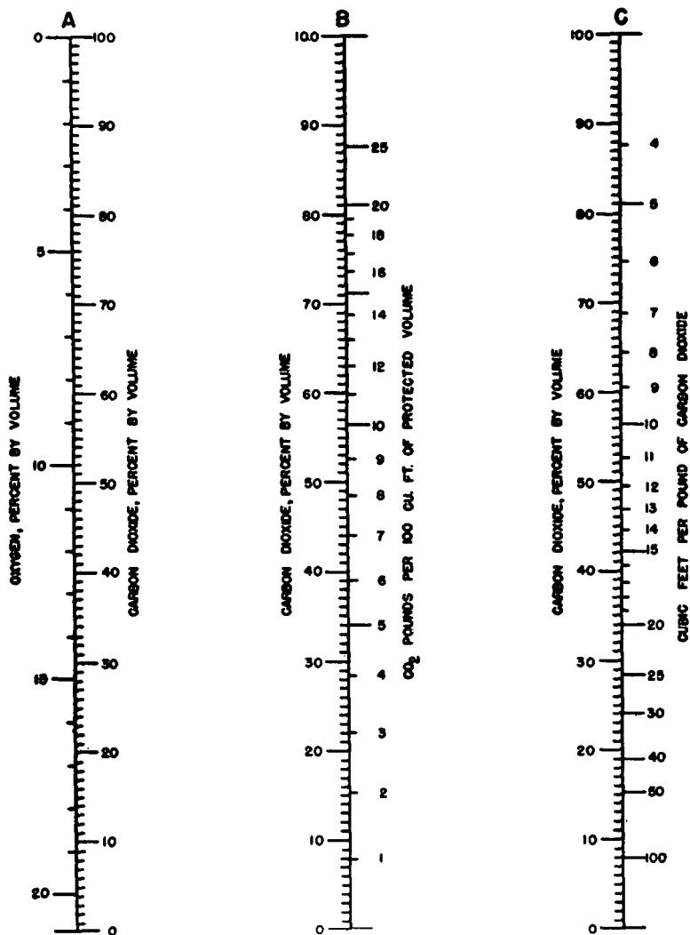
Figure A-7. Carbon dioxide requirement for inert atmospheres, (based on a carbon dioxide expansion of 8.35 cubic feet per pound). Column A shows oxygen content of air-carbon dioxide mixtures; column B shows weight of carbon dioxide in air-carbon dioxide mixtures; column C shows cubic feet per pound of carbon dioxide in air-carbon dioxide mixtures.
