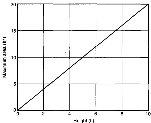
Figure A-3-1(a) Listing or approval curve of a typical nozzle showing maximum area versus height or distance from liquid surface.
