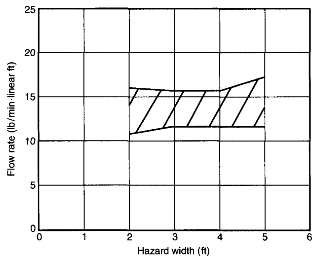
Figure A-3-1(d) Typical listing or approval curve of a linear nozzle showing flow rate versus hazard width.
