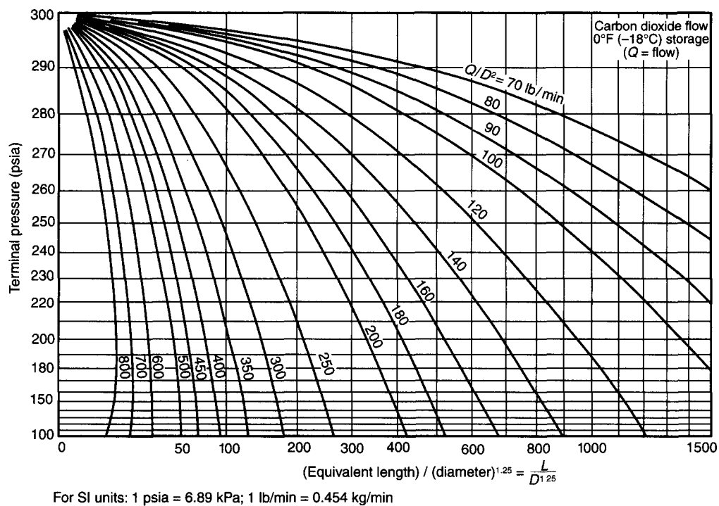
Figure A-1-9.5(a) Pressure drop in pipeline for 300-psia (2068-kPa) storage pressure.
