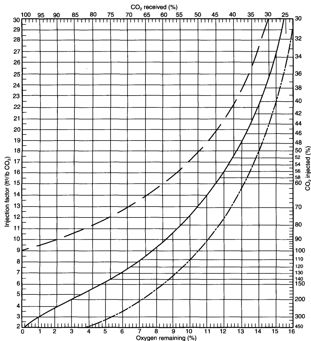
Figure A-2-1(a) Carbon dioxide requirements for inert atmospheres [based on a carbon dioxide expansion of 9 ft³/lb (0.56 m³/kg)]. The top curve (complete displacement) and the bottom curve (no efflux) are theoretical extremes plotted for comparative purposes only. The middle curve (free efflux), the curve to be used, must be tempered by proper safety factors.
