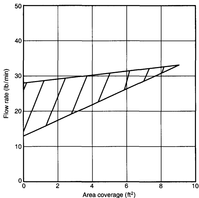
Figure A-3-1(c) Typical listing or approval curve of a tankside nozzle showing flow rate versus area coverage.
