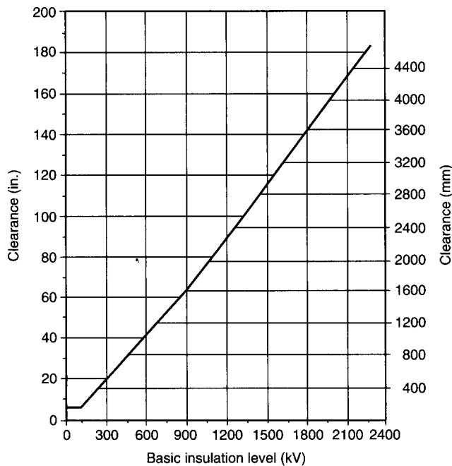
Figure 1-5.2 Clearance from carbon dioxide equipment to live uninsulated electrical components.
