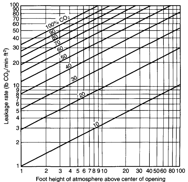
Figure A-2-3(b) Calculated CO 2 loss rate based on an assumed 70°F (21°C) temperature within the enclosure and 70°F (21°C) ambient outside.
