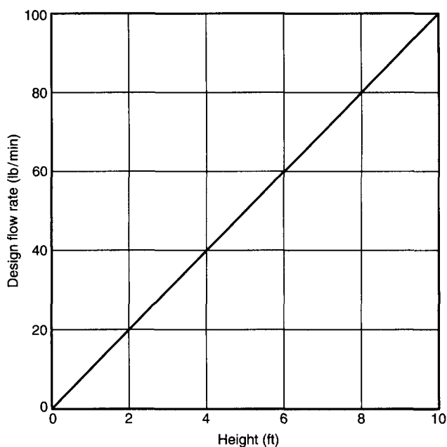
Figure A-3-1(b) Listing or approval curve of a typical nozzle showing design flow rate versus height or distance from liquid surface.
