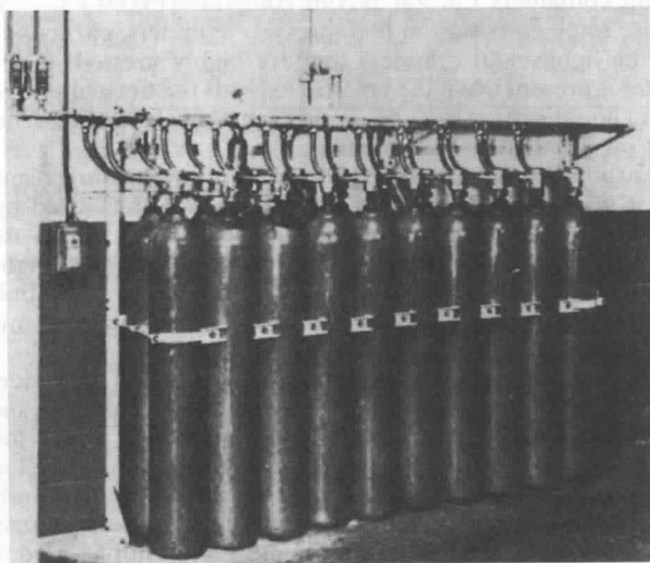
Figure A-1-8.5.1 A typical high-pressure storage facility.
