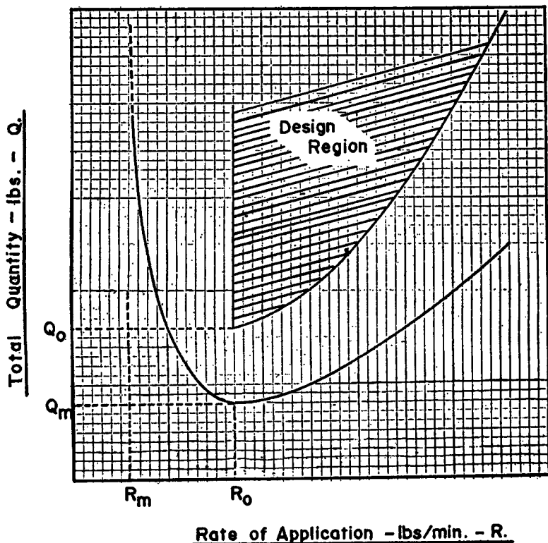
Fig. 4. Typical data presentation for local application nozzles.
