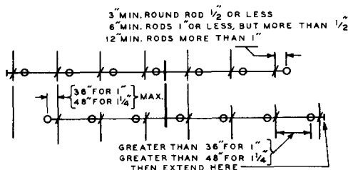
Fig. 3-14.6.3. Distance Sprinkler to Hanger.
