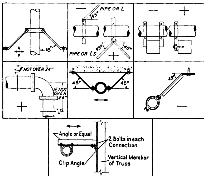
Fig. A-3-10.3.4 Acceptable Types of Sway Bracing.
