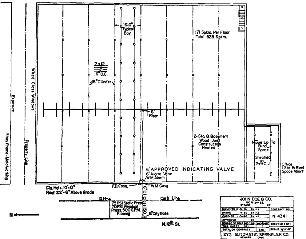
Fig. A-1-9 Typical Preliminary Plan.
