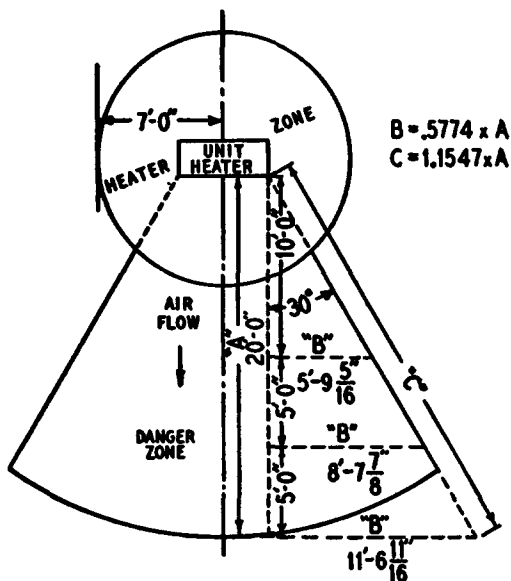
Fig. 3-15.6.4(a). Heater and Danger Zones at Unit Heaters.
