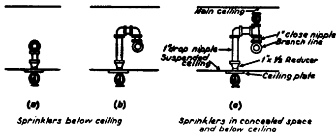
Fig. 3-7.5. Pendent Sprinklers at Suspended Ceiling.
