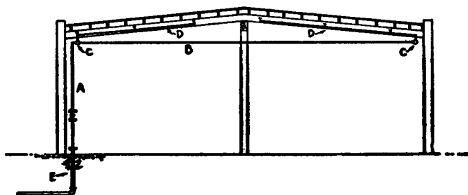
A-3-2 Building Elevation Showing Parts of Sprinkler Piping System. A — Riser; B — Feed Main; C — Cross Main; D — Branch Lines; E — Underground Supply.
