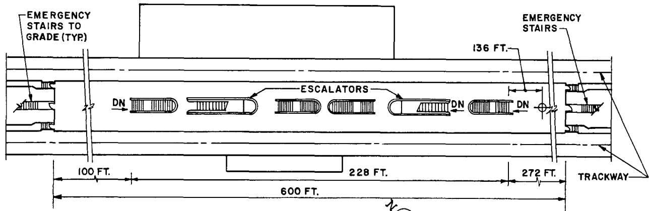
PLATFORM LEVEL PLAN
