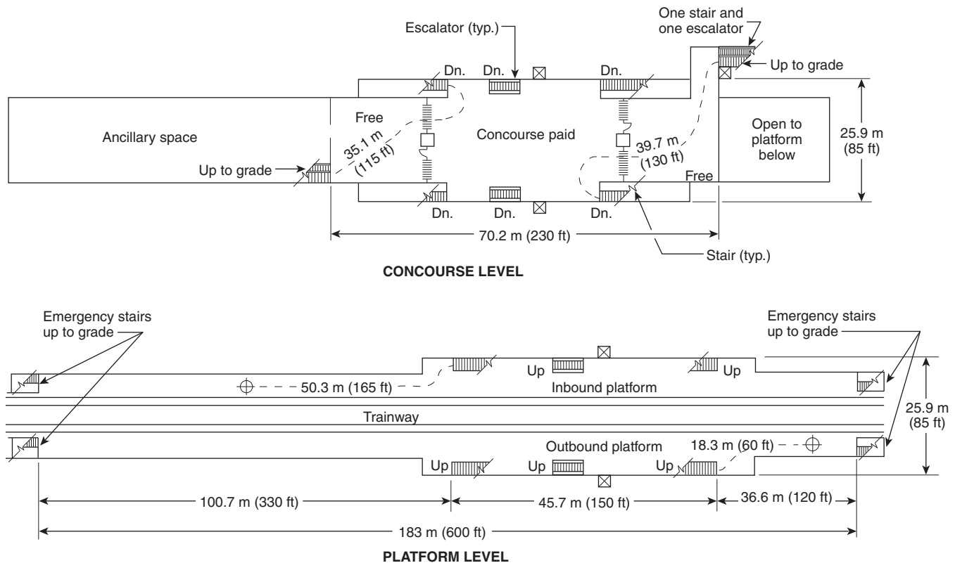
FIGURE C.1.4 Side-Platform Station.
