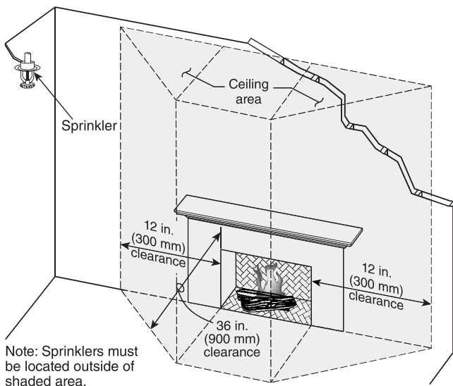
FIGURE A.6.2.3.3.3(b) Recessed Fireplace — Intermediate Temperature Sprinkler Location.
