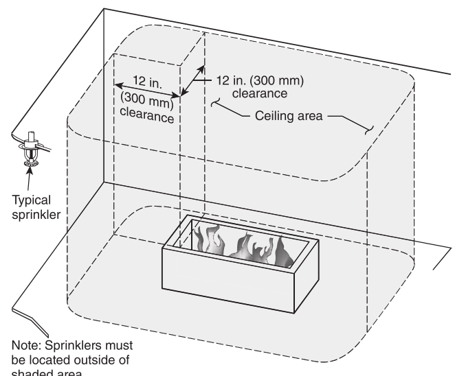
FIGURE A.6.2.3.3.3(d) Open Fireplace — Intermediate Temperature Sprinkler Location.
