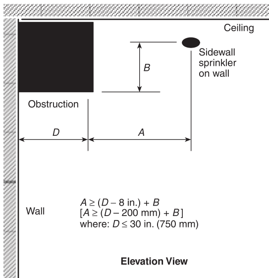
N FIGURE 6.4.6.3.7.2(d) Positioning of Sprinkler to Avoid Obstructions Against Walls — Scenario 2 (Residential Sidewall Spray Sprinklers).
