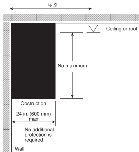
N FIGURE 6.4.6.3.6.3(c) Positioning of Sprinklers to Avoid Obstructions Against Walls — Scenario 3 (Residential Upright and Pendent Spray Sprinklers).
