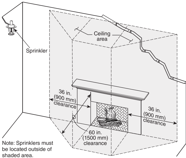
FIGURE A.6.2.3.3.3(a) Recessed Fireplace — Ordinary Temperature Sprinkler Location.
