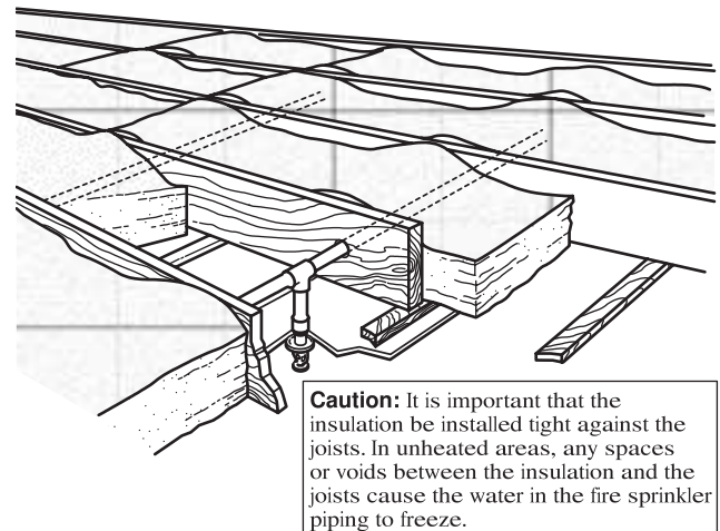
FIGURE A.5.4.2(a) Insulation Recommendations — Arrangement 1.
