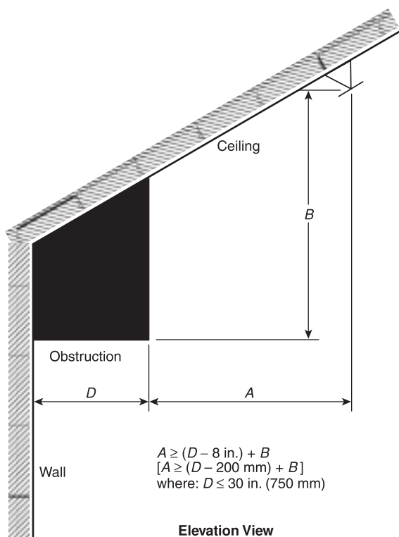
Δ FIGURE 6.4.6.3.6.3(b) Positioning of Sprinkler to Avoid Obstructions Against Walls — Scenario 2 (Residential Upright and Pendent Spray Sprinklers).
