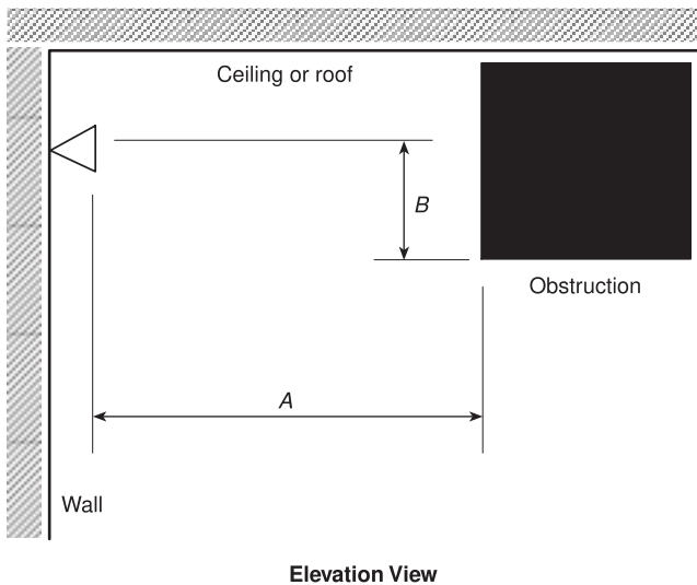
FIGURE 6.4.6.3.7.2(a) Positioning of Sprinkler to Avoid Obstruction (Residential Sidewall Sprinklers).
