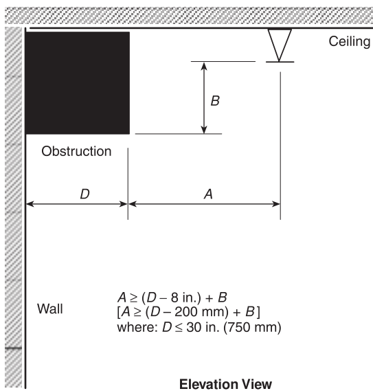
Δ FIGURE 6.4.6.3.6.3(a) Positioning of Sprinkler to Avoid Obstructions Against Walls — Scenario 1 (Residential Upright and Pendent Spray Sprinklers).
