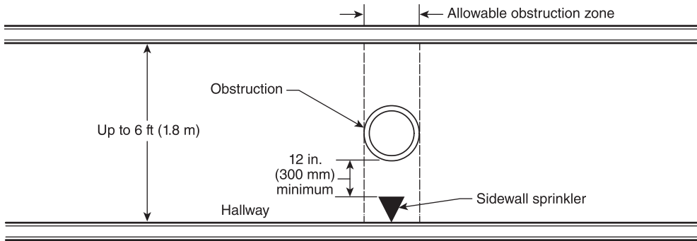
▲ FIGURE 6.4.6.3.5.5 Obstruction in Hallway — Sidewall Sprinkler.
