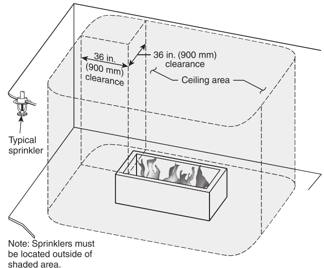
FIGURE A.6.2.3.3.3(c) Open Fireplace — Ordinary Temperature Sprinkler Location.
