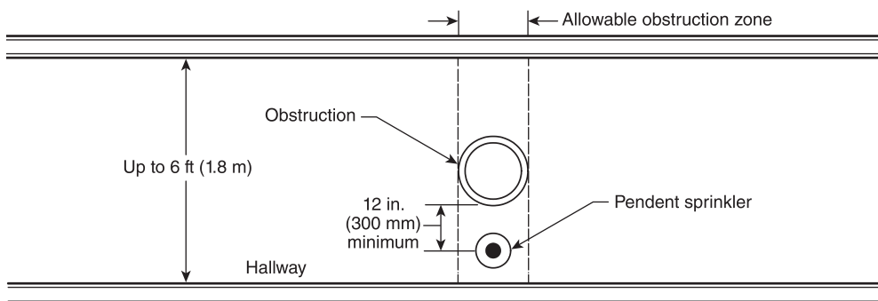
FIGURE 6.4.6.3.4.5 Obstruction in Hallway — Pendent Sprinkler.
