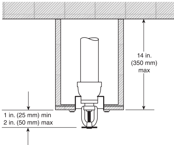
FIGURE 6.4.6.1.1(a) Position of Sprinkler Under a Beam.
