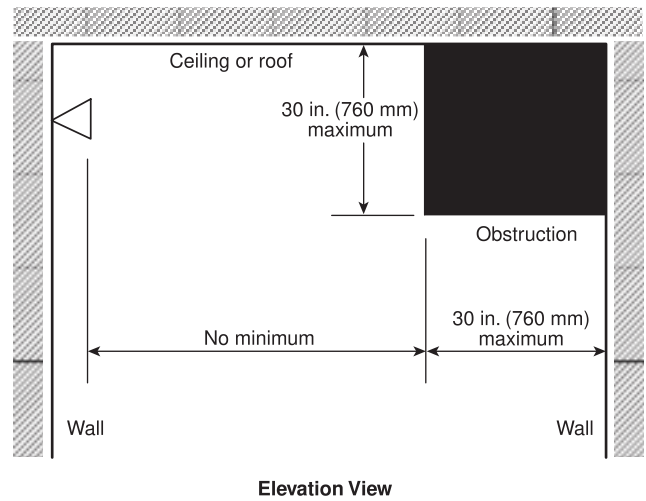
FIGURE 6.4.6.3.7.2(c) Positioning of Sprinkler to Avoid Obstructions Against Walls — Scenario 1 (Residential Sidewall Sprinklers).
