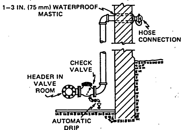
Figure A-5-6.1 Typical fire department connection for wet standpipes.
