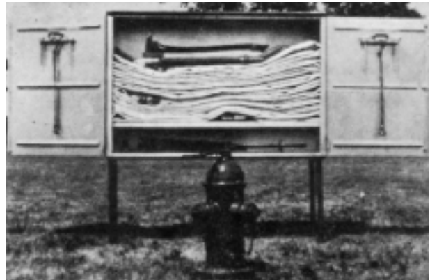
FIGURE A-2-6.2.4(c) This type of hose house can be installed on legs as shown or installed on a wall near, but not directly over, a private hydrant.
