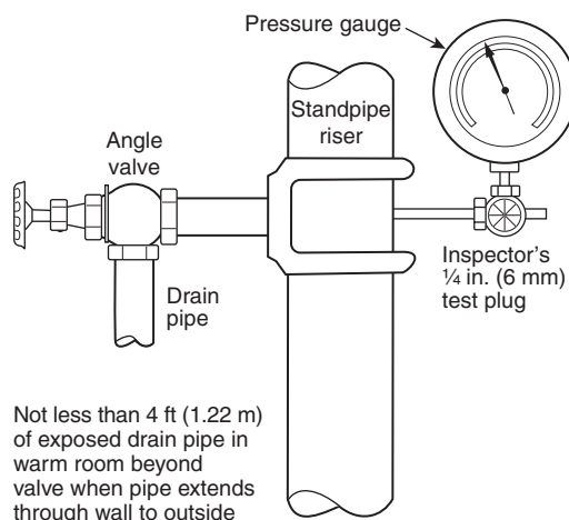
FIGURE 7.11.3 Drain Connection for System Riser.
