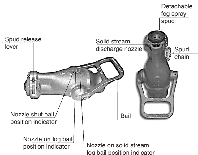
FIGURE 8.3.3.1(c) Navy All-Purpose Nozzle.
