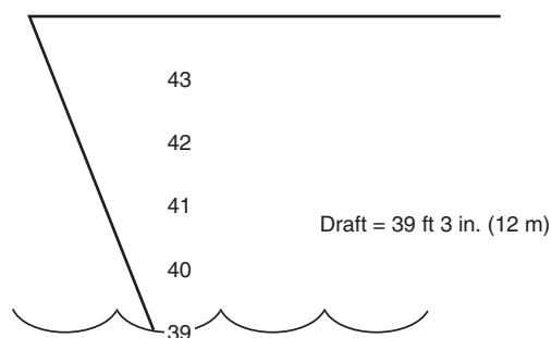
FIGURE 6.10.2.1.1 Draft Marks.
