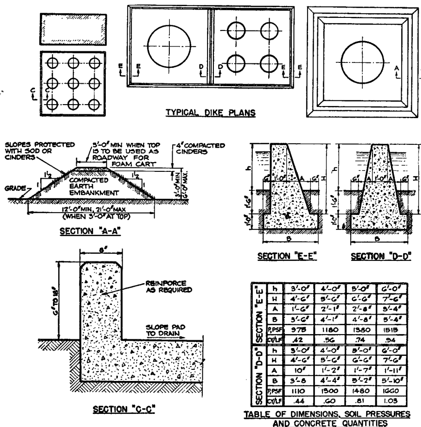
FIG. 4 STANDARD DIKES FOR FIELD STORAGE TANKS
