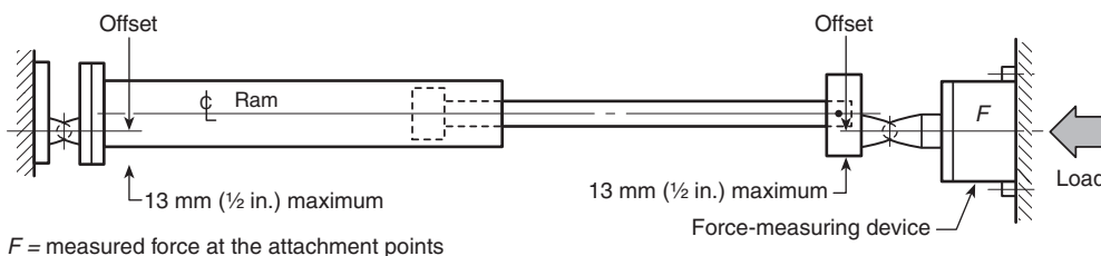
N FIGURE 5.6.12.1 Fixture for Ram Bend Test.
