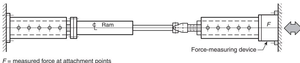
FIGURE 5.6.3.3.1 Test Fixture to Determine Extension and Retraction Forces of Rams.
