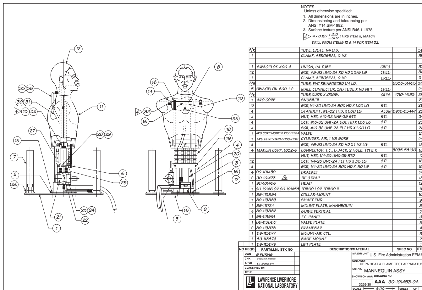
FIGURE 8.11.4.1 Test Mannequin.
