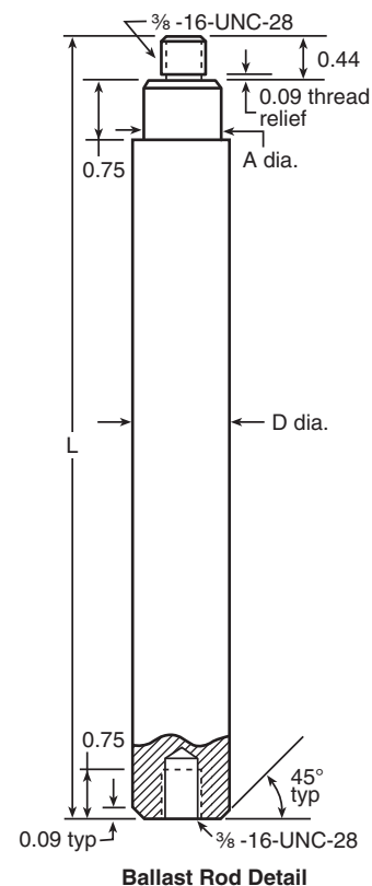
Ballast Rod Detail
