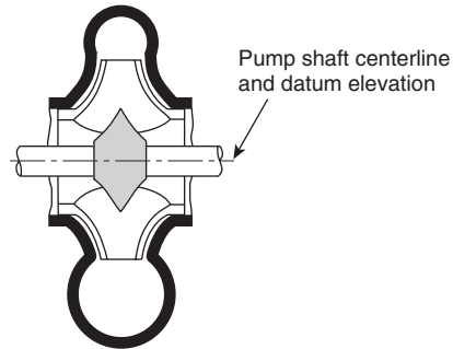
Horizontal double-suction pump
