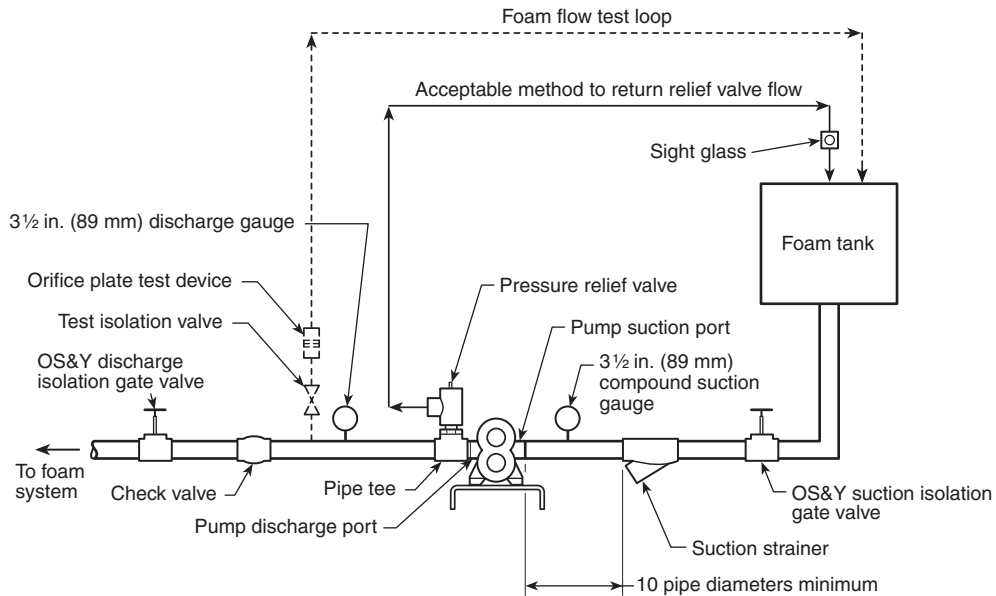
FIGURE A.8.5.2 Typical Foam Pump Piping and Fittings.
