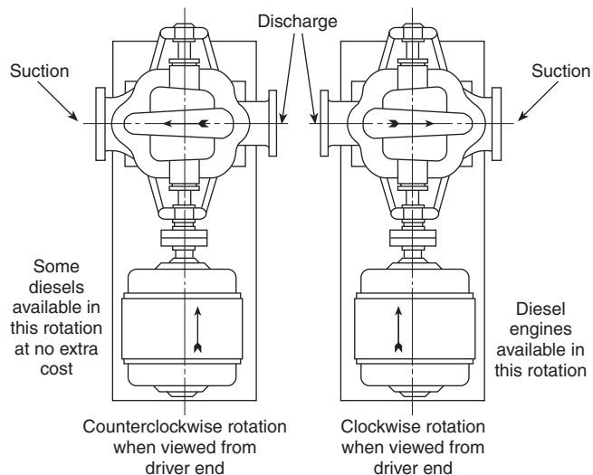
FIGURE A.4.23(a) Horizontal Pump Shaft Rotation.
