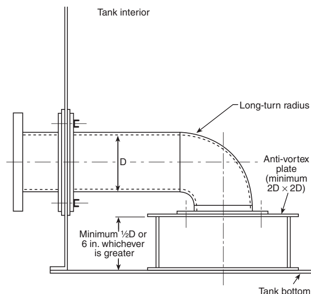
FIGURE A.4.14.10 Anti-Vortex Plate Assembly.
