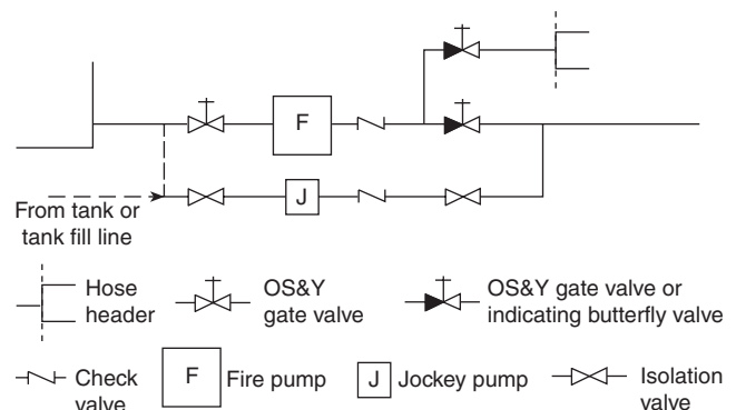
FIGURE A.4.25.5.5 Jockey Pump Installation with Fire Pump.
