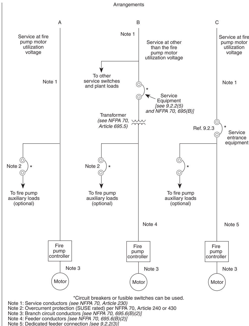
FIGURE A.9.2 Typical Power Supply Arrangements from Source to Motor.
