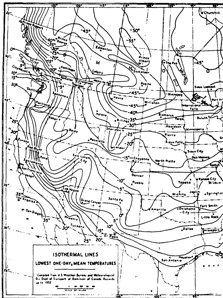
Figure 10-1.4. Isothermal Lines—Lowest One-Day Mean Temperatures (°F).
